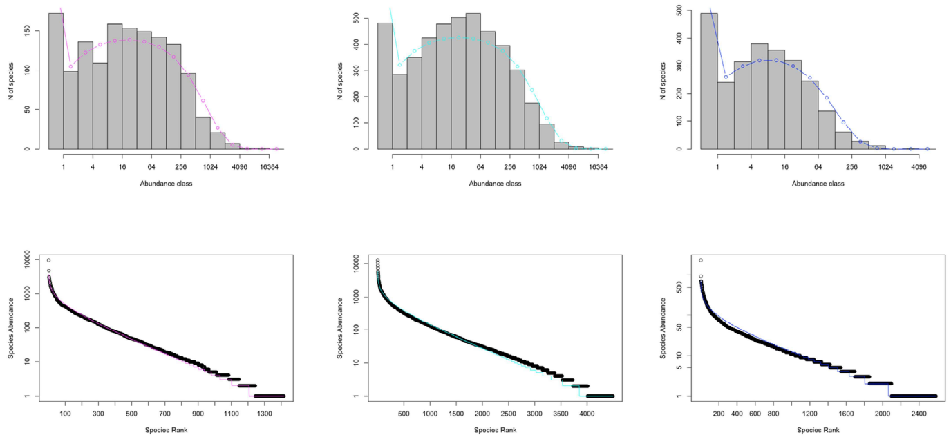
Extended Data Fig. 4 | Preston plots (top row) and rank abundance distributions (bottom row) showing the empirical species abundance distributions for Africa (left) Amazonia (middle) and Southeast Asia (right) with log series fits overlaid. Histogram bars display the empirical species abundance distributions as Preston plots (top row); black markers show the
