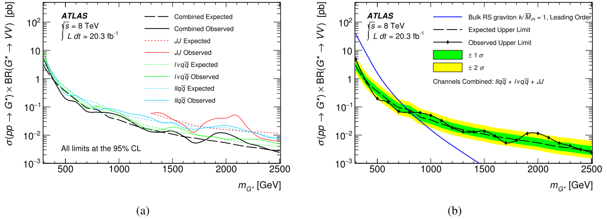
Fig. 4. The 95% CL limits on (a) the bulk G^* using the ll\bar{q}\bar{q} , lv\bar{q}\bar{q} , and JJ channels and their combination, and (b) the combined 95% CL limit with the green (yellow) bands representing the 1\sigma ( 2\sigma ) intervals of the expected limit including statistical and systematic uncertainties. (For interpretation of the references to colour in this figure legend, the reader is referred to the web version of this article.)
