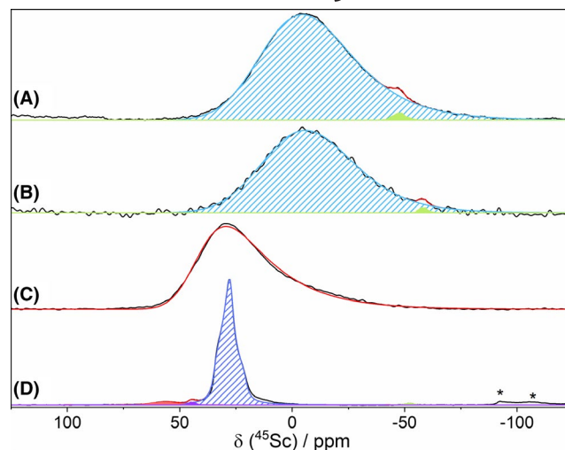
FIGURE 7 ^{45}\text{Sc} MAS NMR experimental spectra (black line) and its numerical deconvolutions (red lines) for samples LSGP (A), LSGP-C-600 (B), LSGP-C-690 (C), and LSGP-C-832 (D). Highlighted curves represent different scandium sites as listed in Table 4. [Color figure can be viewed at wileyonlinelibrary.com ]
