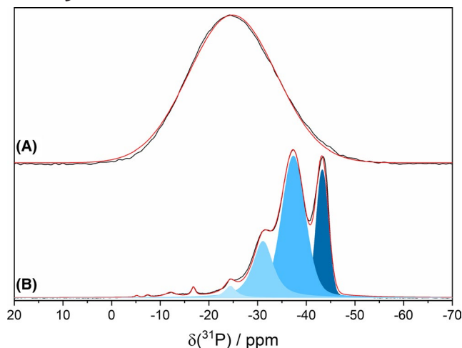
FIGURE 4 ^{31}\text{P} MAS NMR spectra of samples LGGP (A) and LGGP-C-606 (B). Black curves are the experimental data and red curves show the simulations. At (B), \text{P}^{4-}_{(4-n)\text{Ge},n\text{Ga}} units are highlighted in shades of blue and correspond to \text{P}^{4-}_{4\text{Ge},0\text{Ga}} , \text{P}^{4-}_{3\text{Ge},1\text{Ga}} , \text{P}^{4-}_{2\text{Ge},2\text{Ga}} , and \text{P}^{4-}_{1\text{Ge},3\text{Ga}} following the increase of the ppm scale (from dark to light blue). [Color figure can be viewed at wileyonlinelibrary.com ]
