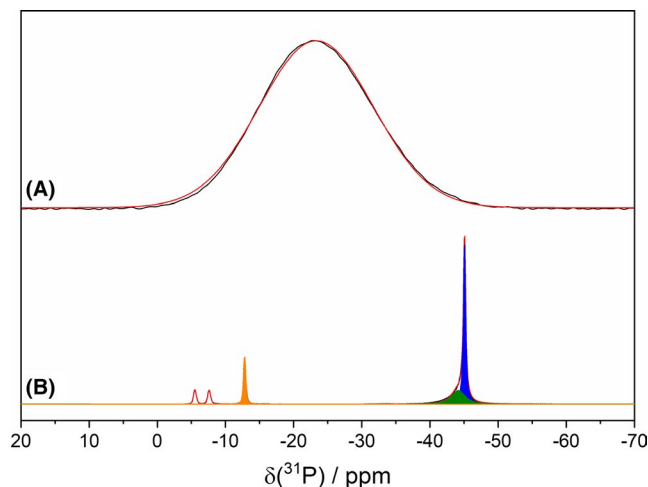
FIGURE 6 ^{31}\text{P} MAS NMR spectra of samples LYGP (A) and LYGP-C-728 (B). At (B), different phosphate units are highlighted in blue (highly crystalline \text{P}_{4\text{Ge},0\text{Y}}^4 ), green ( \text{P}_{4\text{Ge},0\text{Y}}^4 ), and orange ( \text{YPO}_4 ). Unfilled curves are assigned to P1 units in \text{Li}_4\text{P}_2\text{O}_7 (phosphate units with only one bridging oxygen). Red curves represent simulated spectra. [Color figure can be viewed at wileyonlinelibrary.com ]
