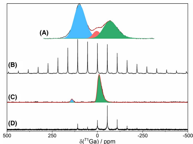
FIGURE 8 ^{71}\text{Ga} MAS (A,C) and QCPMG (B,D) NMR spectra of samples LSGP and LSGP-C-606 (black line) and their deconvolution (red curve in A). Four-, five-, and six-coordinated gallium resonances are highlighted in blue, red and green respectively in A and C. [Color figure can be viewed at wileyonlinelibrary.com]
