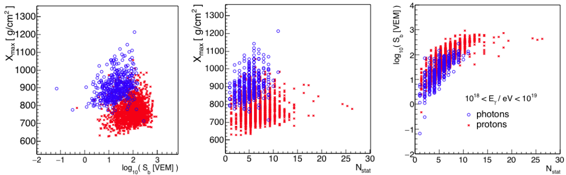
Figure 1: Correlation between the discriminating observables used in the MVA for the energy range 10^{18} < E_\gamma < 10^{19}\text{eV} [5]: the simulated photon sample is shown as blue circles, while the proton sample is denoted by red stars.
