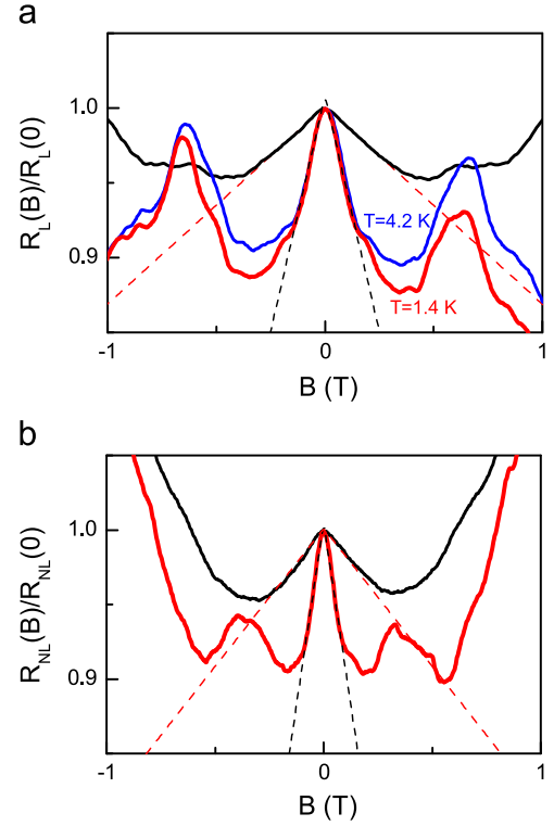
Fig. 4. (Color online) (a) The relative local resistance R_l(B)/R_l(0) ( R_l = R_{l=1.4; V=2.3} ) as a function of the magnetic field for the two values of the gate voltage V_g - V_{CNP} (V): 0.35 (black), 0.53 (blue, red), and two temperatures (device B). (b) The relative nonlocal resistance R_{NL}(B)/R_{NL}(0) ( R_{NL} = R_{l=2.6; V=3.5} ) as a function of the magnetic field for the two values of the gate voltage V_g - V_{CNP} : 0.35 (black), 0.5 (red) (device A). Dashed lines are B-linear approximations.
