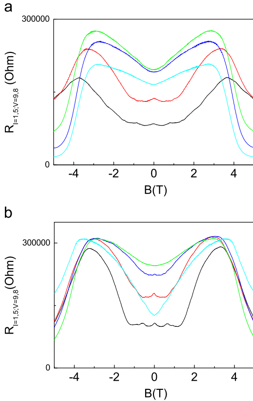
Fig. 3. (Color online) The local resistance R for two samples with multiterminal configuration (devices B) as a function of the magnetic field for the different values of the gate voltages, when the Fermi energy passes through CNP from the hole to electronic side of the resistance peak. (a) V_g - V_{CNP} (V): -0.15 (cyan), -0.02 (blue), 0.1 (green), 0.35 (red), 0.47 (black). (b) V_g - V_{CNP} (V): -0.18 (cyan), 0.05 (green), 0.25 (blue), 0.37 (red), 0.45 (black).
