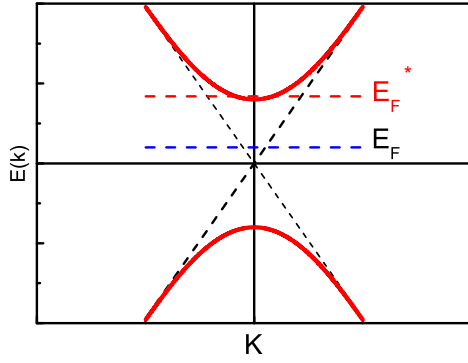
Fig. 1. (Color online) Schematic of the energy spectrum of 2D TI near k=0 . Solid lines -spectrum for the bulk electrons, dashes- helical edge state spectrum. Positions of the Fermi energy in the bulk gap and near the bottom of the conductive bands are indicated.
