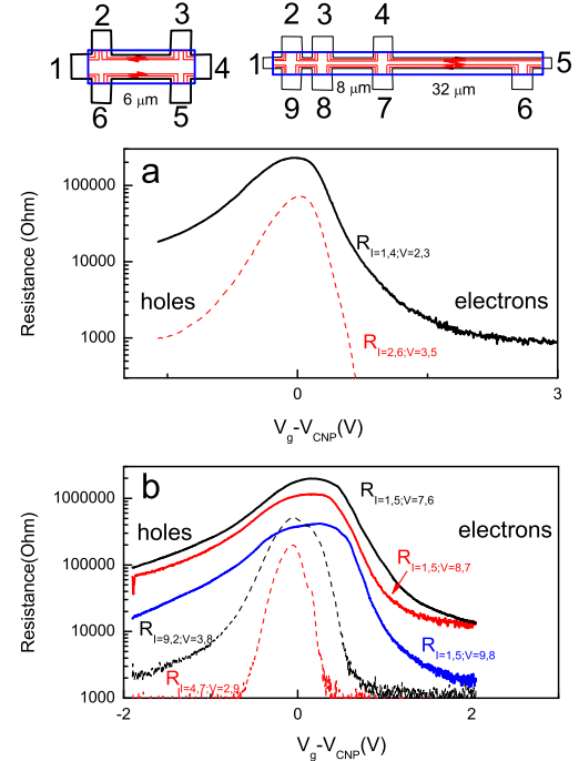
Fig. 2. (Color online) (a) The local and nonlocal resistances R as a function of the gate voltage at zero magnetic field measured by various voltage probes for samples A (a) and B (b), T=4.2 K. Top panel-shows schematic view of the samples. The perimeter of the gate is shown by blue rectangle.
