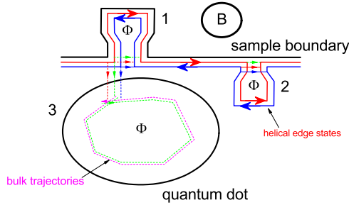
Fig. 6. (Color online) Schematics of helical edge state propagation along a disordered edge in 2DTI in a perpendicular magnetic field. Electrons tunnel in and out quantum dot (puddle) created by inhomogeneous charge distribution. Electron helical trajectories form loops resulted from the edge roughness (1), near bulk disorder (2) and metallic puddles (3). Bulk electron trajectories form loops inside of the puddle.
