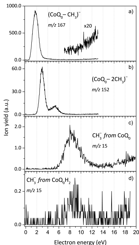
Figure 7. Anion efficiency curves as a function of the electron energy for the formation of the following fragment anions: a) (\text{CoQ}_0\text{--CH}_3)^- from \text{CoQ}_0 , the inset (x20) shows the signal for ion-pair formation; b) (\text{CoQ}_0\text{--}2\text{CH}_3)^- ; c) \text{CH}_3^- from \text{CoQ}_0 and d) \text{CH}_3^- from \text{CoQ}_0\text{H}_2 .
