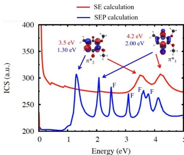
Figure 4. Integral cross section (ICS) for elastic electron scattering by the \text{CoQ}_0 molecule. The red and blue lines correspond, respectively, to the results obtained in the SE and SEP approximations. Virtual orbitals associated with the shape resonances ( \pi_2^* and \pi_3^* ) are also shown. The arrows connect these plots to the SE and SEP level peaks arising from those anion states, and the peak positions in both approximations are indicated alongside the orbital plots. In the SEP cross section, we also assign the peaks around 2.50 eV, 3.08 eV, 3.61 eV and 3.78 eV to Feshbach (F) resonances.
