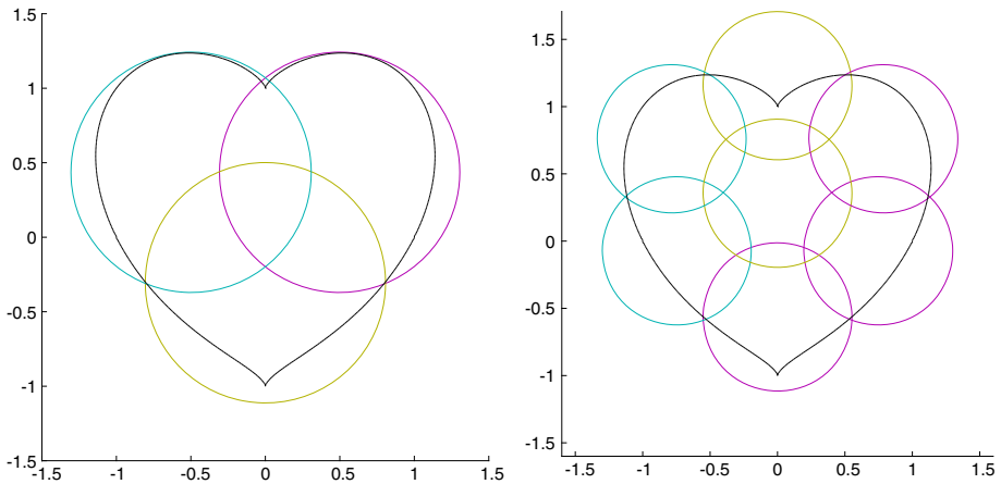
Fig. 2 Solution found by an inexact restoration method for covering a heart-shaped object
