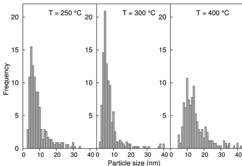
Fig. 4. Particle size histograms obtained from the transmission electron micrographs of the \text{NiFe}_2\text{O}_4 nanoparticle powder for samples synthesized at 250 °C, 300 °C and 400 °C.
