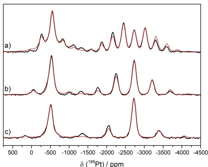
Figure 9. ^{195}\text{Pt} MAS-NMR spectra (black trace) of \text{Sr}_2\text{Pt}_3\text{Al}_8 at B_0 = 5.64\text{ T} and three different spinning speeds a) 15.0 kHz, b) 25.0 kHz, c) 35.0 kHz. Simulations of the spinning sideband manifold are shown as red traces, based on the magnetic shielding tensor components described in the text.
