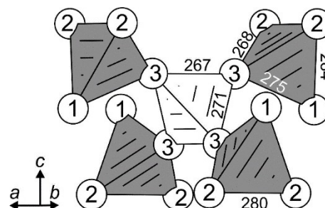
Figure 1. (Al_4)_5 supertetrahedra in Sr_2Pt_3Al_8 . Interatomic distances are given in pm.
