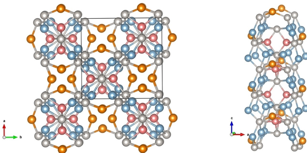
Figure 10. Pt–Al network in \text{Sr}_2\text{Pt}_3\text{Al}_8 . Perspective view along the crystallographic c axis (left), and one tube of the network in the c direction (right). Pink, blue, orange, and gray spheres represent Al1, Al2, Al3 and Pt atoms.
