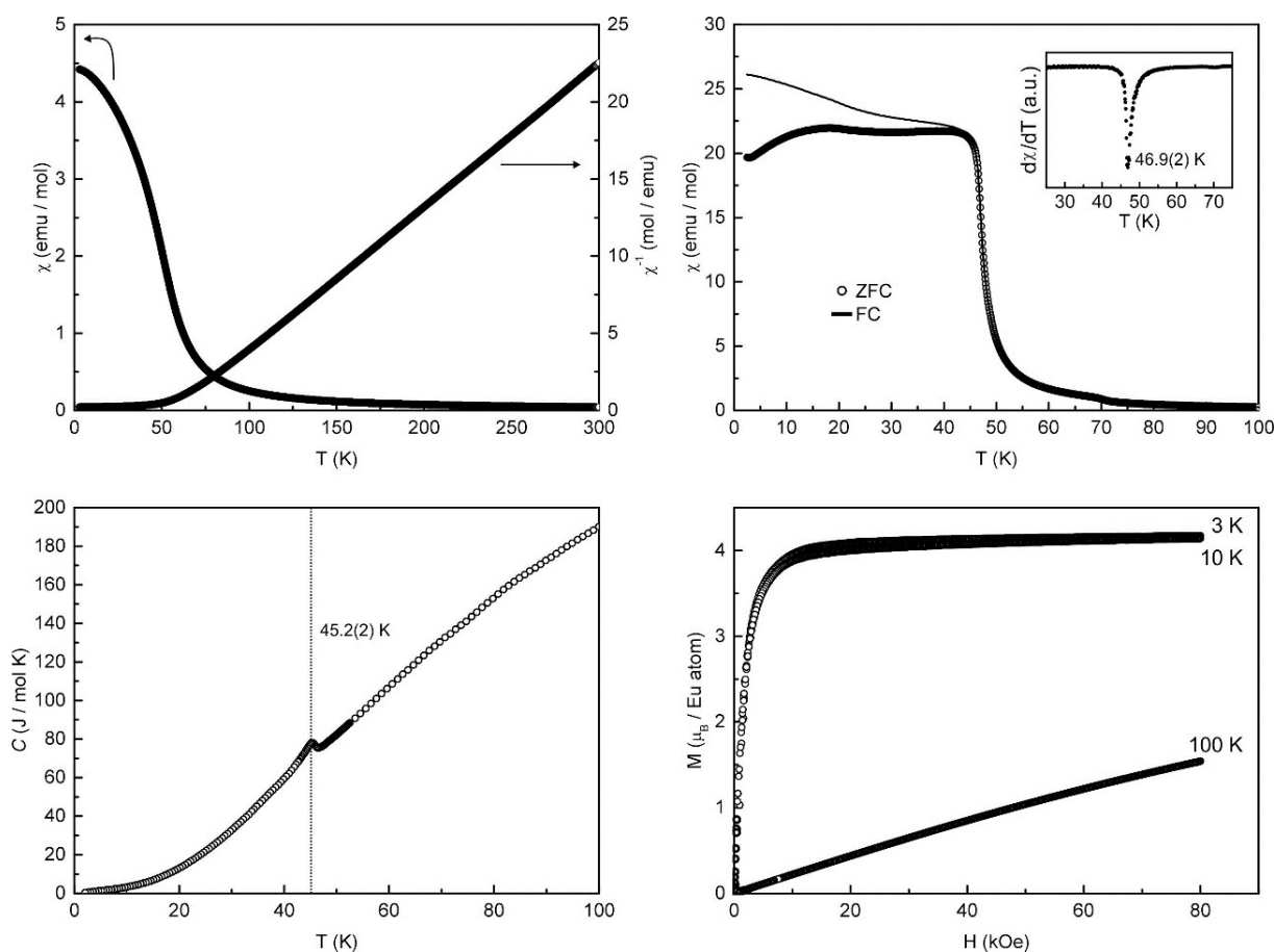
Figure 6. Magnetic properties of \text{Eu}_2\text{Ni}_8\text{Si}_3 : (top left) temperature dependence of the magnetic susceptibility \chi and its reciprocal \chi^{-1} measured at an applied external field of 10 kOe; (top right) magnetic susceptibility in zero-field-cooled (ZFC) and field-cooled (FC) mode at 100 Oe, the inset depicts the derivative d\chi/dT ; (bottom left) temperature dependence of the specific heat capacity; (bottom right) magnetization isotherms, recorded at 3, 10, and 100 K.
