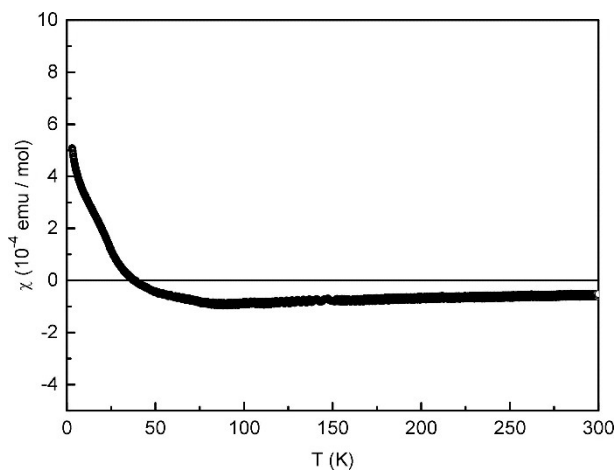
Figure 5. Temperature dependence of the magnetic susceptibility \chi of \text{Sr}_2\text{Pt}_3\text{Al}_8 , measured in zero-field-cooled (ZFC) mode at 10 kOe.
