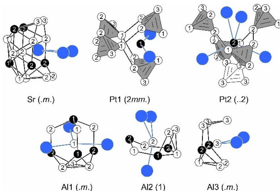
Figure 3. Coordination environments of the crystallographically independent sites in \text{Sr}_2\text{Pt}_3\text{Al}_8 with additional point symmetries given. Sr, Pt and Al atoms are depicted as blue, black and open white circles, respectively.
