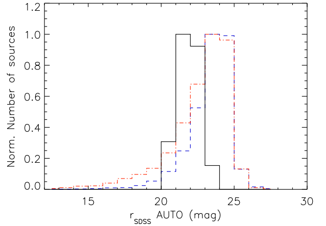
Fig. 5. Histogram of the r_{SDSS} (AUTO photometry) magnitude of our selected candidates (black line). Blue and red histograms correspond to the total sample of galaxies and stars in the miniJPAS dual catalogue, respectively, classified taking into account the miniJPAS stellarity index. The three histograms are normalized to the peak of each distribution.
