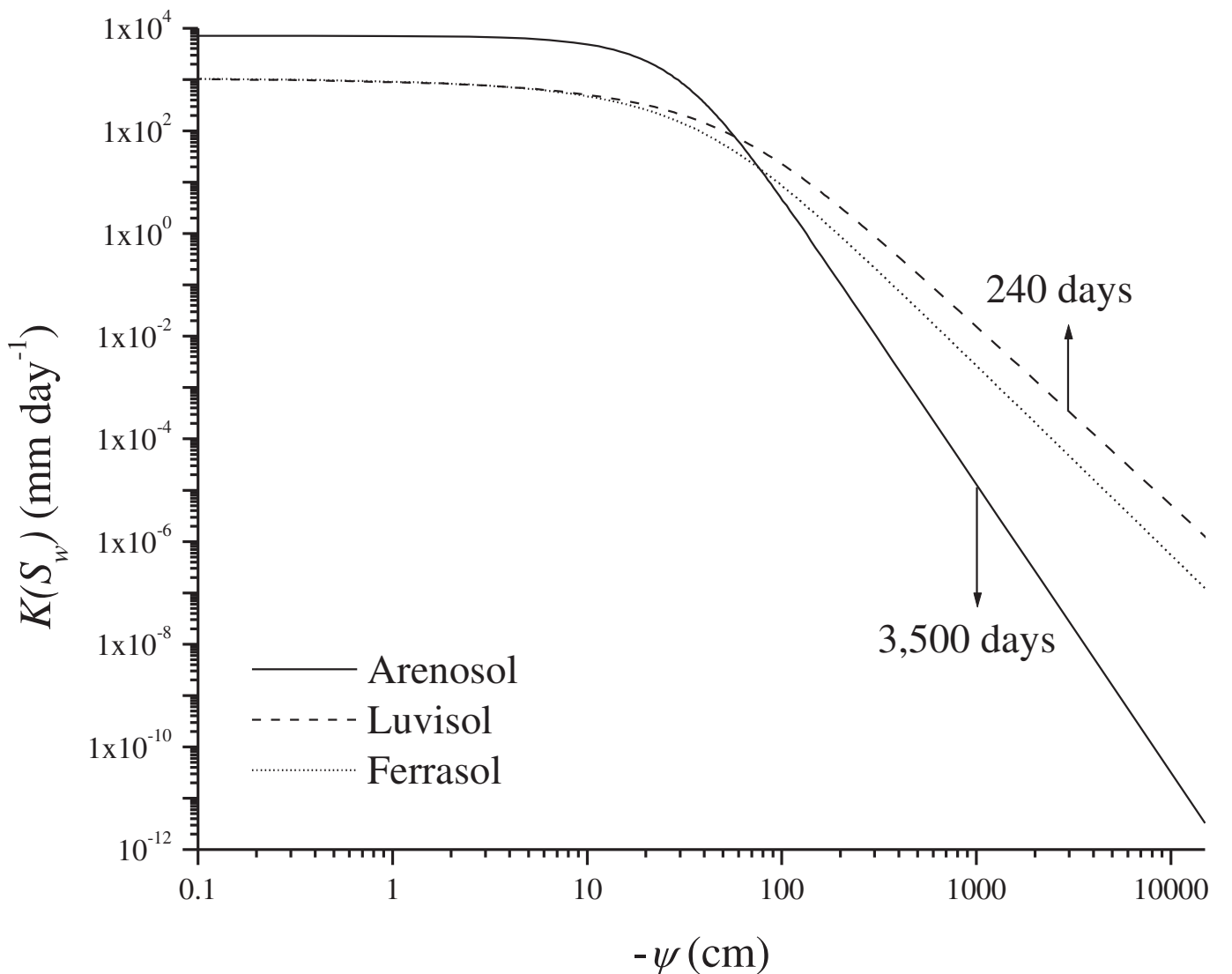
Fig. 6. Predicted hydraulic conductivity curves versus pressure head ( \Psi ) using the Mualem model and van Genuchten parameters obtained by fitting the conventional SWRC data with Eq. (4) for Arenosol, Luvisol and Ferrasol showed in Fig. 5. The arrows indicate the time necessary for a reduction of 1 % in the water saturation at the corresponding \Psi , using \frac{dS_w}{dt} = \frac{K(S_w)}{z\phi^2} (Ghanbarian and Hunt, 2017).
