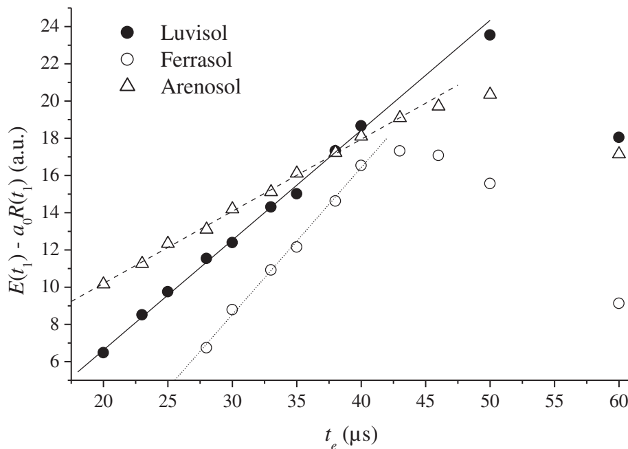
Fig. 2. Optimisation of the encoding time ( t_e ) for the studied soils. The signal amplitude, after removing the ground mode T_1 contribution by Eq. (2) ( S ), linearly increased up to t_e = 40 \mu\text{s} for all the studied samples. E(t_1) and R(t_1) are the initial amplitude of the E and R decays, respectively; a_0 is the scaling factor; and a.u. is arbitrary units.
