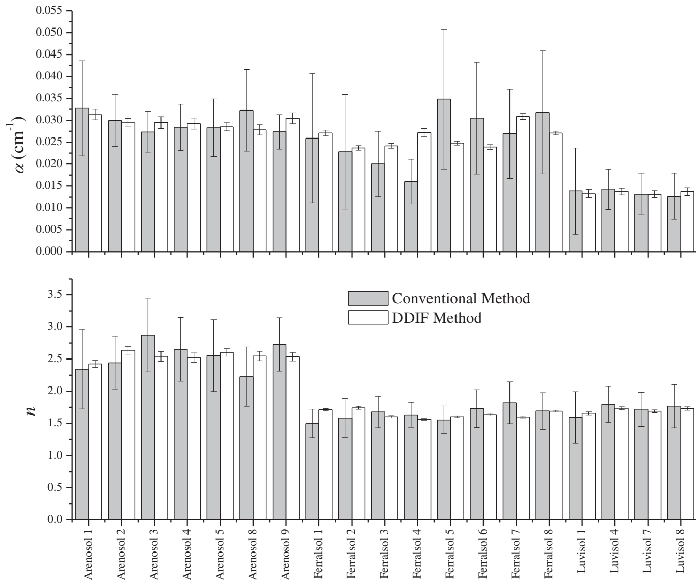
Fig. 10. Adjusted van Genuchten parameters from SWRC obtained by the conventional (tension table and pressure plate extractor) and DDIF methods after the shift of the matric potential (the minimum matric potential in the DDIF experiment for the Arenosol was \psi = -1,000 cm), the bars are the 95 % Confidence Intervals of the fitted parameters.
