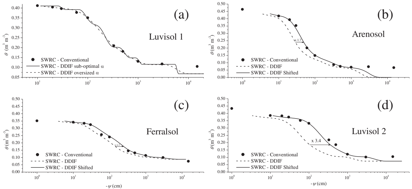
Fig. 5. Typical SWRC estimated from pore size distribution obtained from DDIF experiment (lines) compared to SWRC obtained by the conventional method using tension table and pressure plate extractor (black bullets). (a): The solid line is the SWRC obtained from the DDIF method with a sub-optimal Tikhonov regularisation while the dashed one is with the oversized Tikhonov regularisation. (b-d): The dashed line is the SWRC obtained directly from the pore size distribution from the DDIF method while the solid one is the same curve after shifting the \Psi_m scale by a factor of 1.7 (Arenosol and Ferrasol) or 3.4 (Luvisol). These factors were obtained after calibration against the \Psi_m of the reference method at -100 cm (Costabel and Yaramanci, 2013). The same graphs for all the analysed samples can be found in the Supplementary material (Fig. S3).
