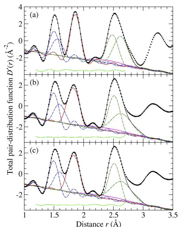
FIG. 16. The fitted D'(r) functions for (a) crystalline, (b) as-prepared glassy, and (c) annealed glassy ( T_{\text{TT}} = 873 K) NAGP with x = 0 measured using D4c. The filled circles give the measured function; the black solid curve gives the fitted function; and the other curves show the contributions from the P–O (blue broken curves), Ge–O (red solid curve), Na–O (magenta solid curve), and O–O (green broken curves) correlations. The displaced green solid curve shows the residual. For the glass, the Na–O and O–O correlations are introduced to constrain the peaks fitted at smaller r -values.
