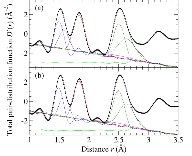
FIG. S2. The fitted D'(r) functions measured using D4c for NAGP with x = 0 annealed at T_{\text{TT}} = 876 K for either (a) 0.25 h or (b) 0.5 h. In a given panel, the filled circles give the measured function, the black solid curve gives the fitted function, and the other curves show the contributions from the P-O (blue broken curves), Ge-O (red solid curve), Na-O (magenta solid curve) and O-O (green broken curves) correlations. The displaced green solid curve shows the residual. The Na-O and O-O correlations are introduced to constrain the peaks fitted at smaller r -values.
