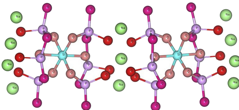
FIG. 24. Two of the [\text{Si}^{(6)}\text{P}_6^{(3)}\text{O}_{10}\text{O}_6]^{2-} super-structural units in the model of Ren and Eckert 66 for glassy \text{Na}_2\text{P}_6\text{SiO}_{18} , where charge-shuttling ensures that the NBO atoms in the \text{P}^{(3)} phosphate motifs carry a partial negative charge. Other super-structural units (not shown) ensure that the top and bottom rows of \text{Na}^+ ions have a 1/4 share in each unit and that the remaining \text{Na}^+ ions have a 1/2 share in each unit. The charge of -4e on the illustrated units is therefore balanced by the net charge of (5e \times 1/2) + (6e \times 1/4) = +4e on the illustrated \text{Na}^+ ions. Reprinted with permission from J. Ren and H. Eckert, J. Phys. Chem. C 122 , 27620 (2018). Copyright 2018, American Chemical Society.
