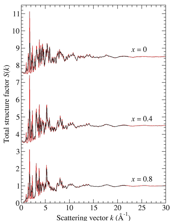
FIG. 9. The total structure factors S(k) for crystalline NAGP with x = 0, 0.4 , and 0.8 measured using GEM (red curves) or D4c (black curves). The vertical error bars are smaller than the line thickness at most k values. For clarity of presentation, several of the curves are displaced vertically and the GEM datasets are shown only to 30 \text{ \AA}^{-1} .
