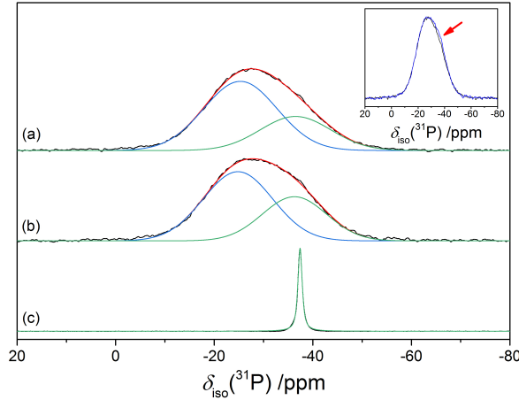
FIG. S1. The single-pulse ^{31}\text{P} MAS NMR spectra (black curves) measured for (a) as-prepared glassy, (b) annealed glassy and (c) crystalline NAGP with x = 0 . In (a) and (b) the spectra are fitted to two Gaussian peaks (blue and green curves) with an approximately 2:1 ratio of areas. The sum of fitted functions is given by the red curve. In (c) the spectrum is fitted to a Gauss-Lorentz curve. The inset shows an overlay of the spectra in (a) and (b) given by the black and blue curves, respectively, where the arrow points to a small but discernible change of intensity on annealing the glass.
