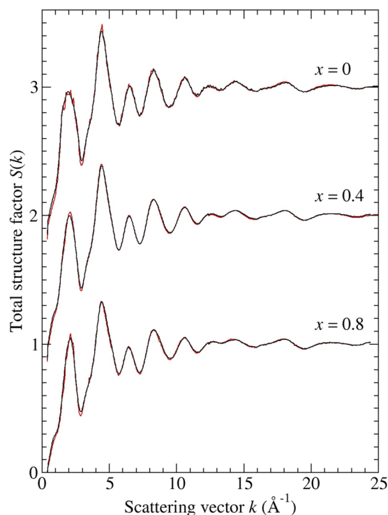
FIG. 12. The total structure factors S(k) for the as-prepared (black curves) vs annealed (red curves) glassy NAGP with x = 0, 0.4 , and 0.8 measured using XRD. Several of the curves are displaced vertically for clarity of presentation.
