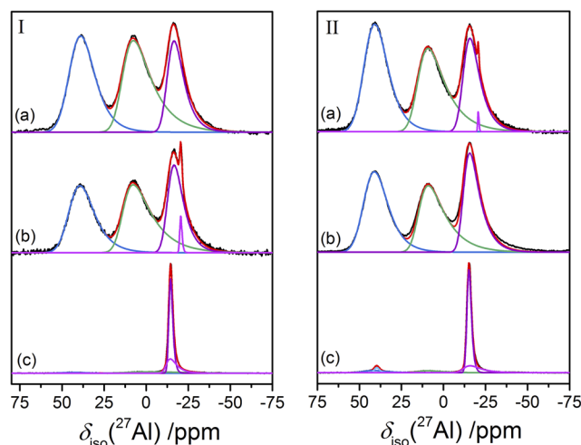
FIG. 8. The single-pulse ^{27}\text{Al} MAS NMR spectra (black curves) measured for (a) as-prepared glassy, (b) annealed glassy, and (c) crystalline NAGP with (I) x = 0.4 or (II) x = 0.8 . The Cjzek fits to the spectral components are given by the blue or cyan curves for Al(IV), the green curve for Al(V), and the violet or magenta curves for Al(VI). The sum of fitted functions is given by the red curve.
