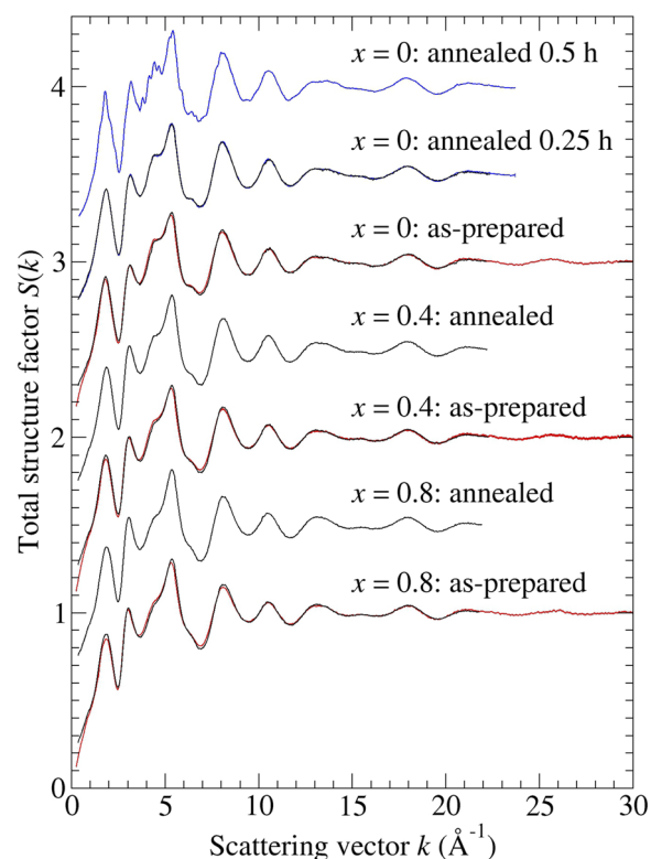
FIG. 10. The total structure factors S(k) for as-prepared vs annealed glassy NAGP with x = 0, 0.4 , and 0.8 . The red curves give the GEM datasets, and the black or blue curves give the D4c datasets, where the latter correspond to the x = 0 glass annealed at T_{\text{T}} = 876 \text{ K} for either 0.25 or 0.5 \text{ h} . The vertical error bars are smaller than the line thickness at most k values. For clarity of presentation, several of the curves are displaced vertically and the GEM datasets are shown only to 30 \text{ \AA}^{-1} .
