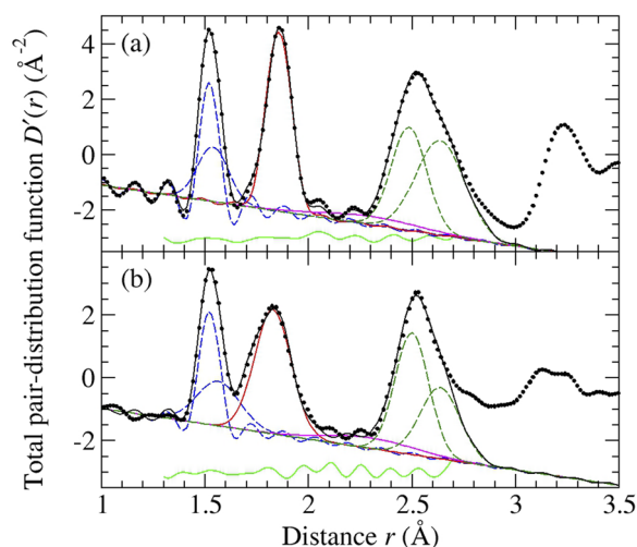
FIG. 14. The fitted D'(r) functions for (a) crystalline and (b) as-prepared glassy NAGP with x = 0 measured using GEM. The filled circles give the measured function; the black solid curve gives the fitted function; and the other curves show the contributions from the P–O (blue broken curves), Ge–O (red solid curve), Na–O (magenta solid curve), and O–O (green broken curves) correlations. The displaced green solid curve shows the residual. For the glass, the Na–O and O–O correlations are introduced to constrain the peaks fitted at smaller r -values.
