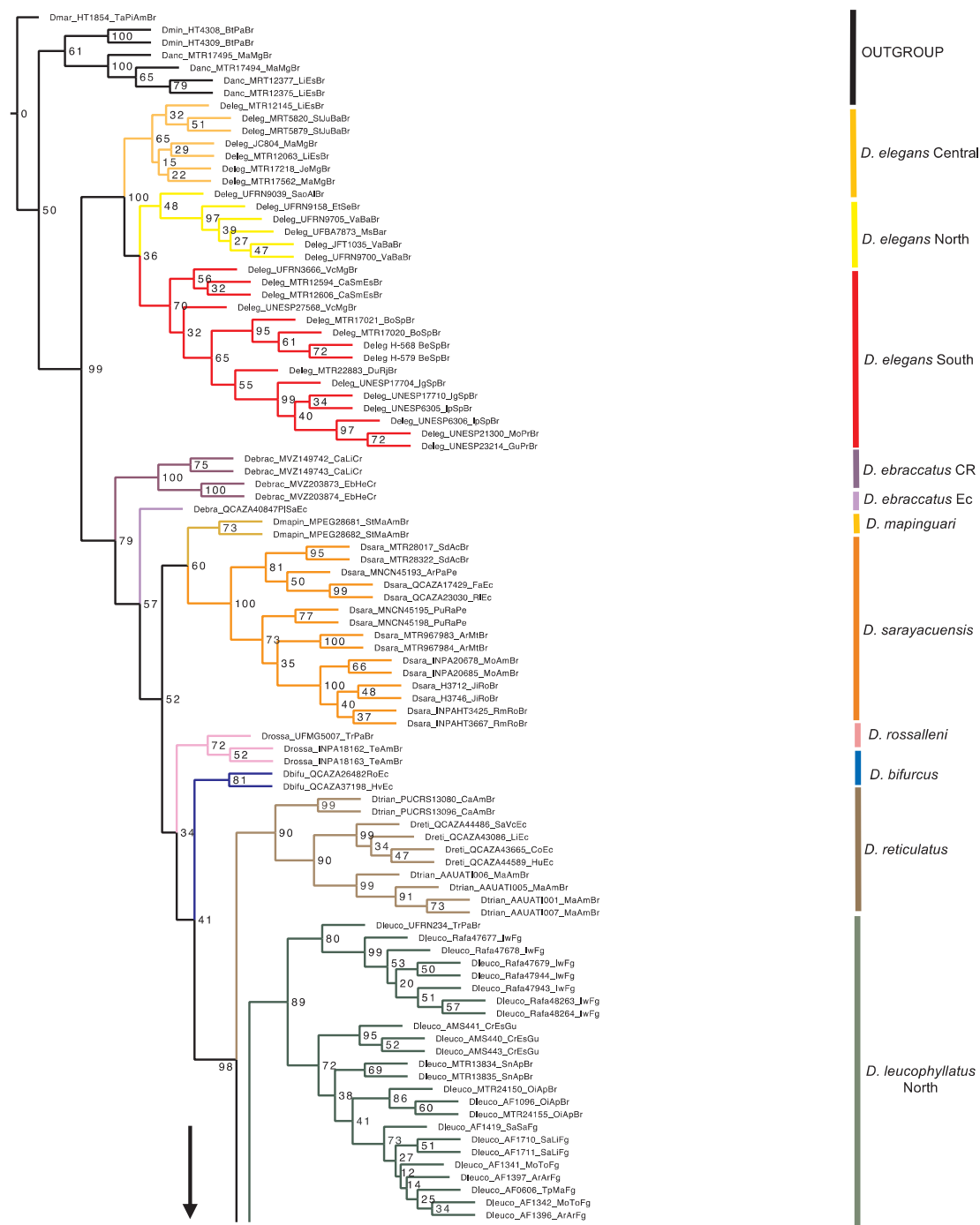
Fig. 2. Molecular phylogeny of sampled individuals from the Dendropsophus leucophyllatus species group based on SVDQuartets analysis from 4,048 unlinked SNPs. Clade colors correspond to the topology used for defining the lineages tree at SNAPP analysis. Scale bar represents estimated substitution per site. Posterior probability values for all nodes are based on 100 bootstrap pseudoreplicates.
