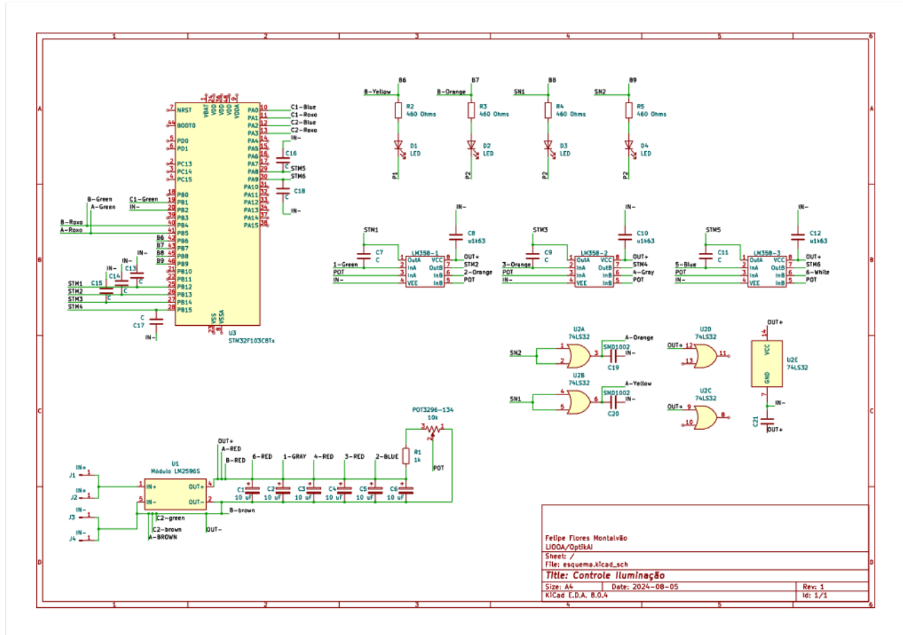
Figure 1. Illumination Control System with STM32 BluePill
