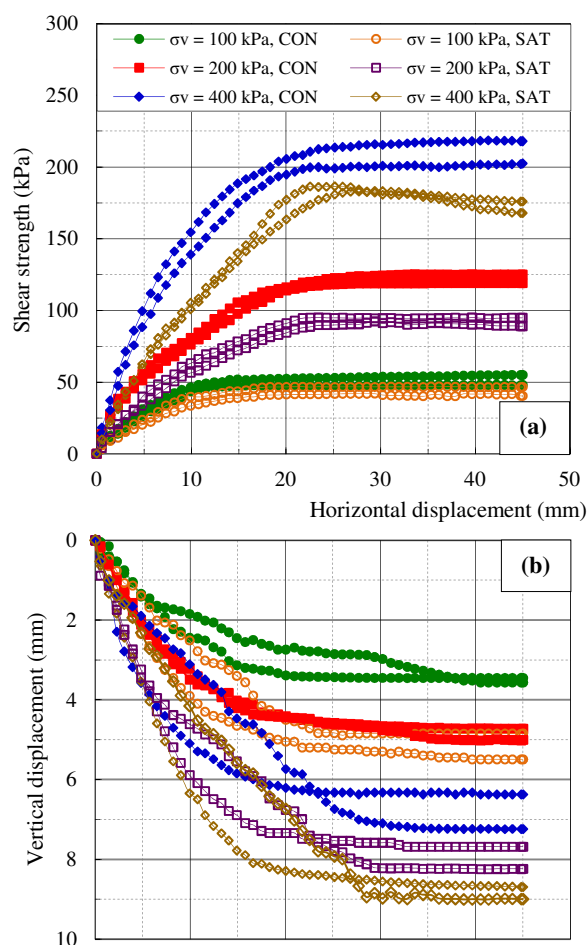
Fig. 5. Direct shear results of silty sand samples for e_i = 1.0 : effect of test condition on (a) shear strength; (b) volumetric behaviour.
