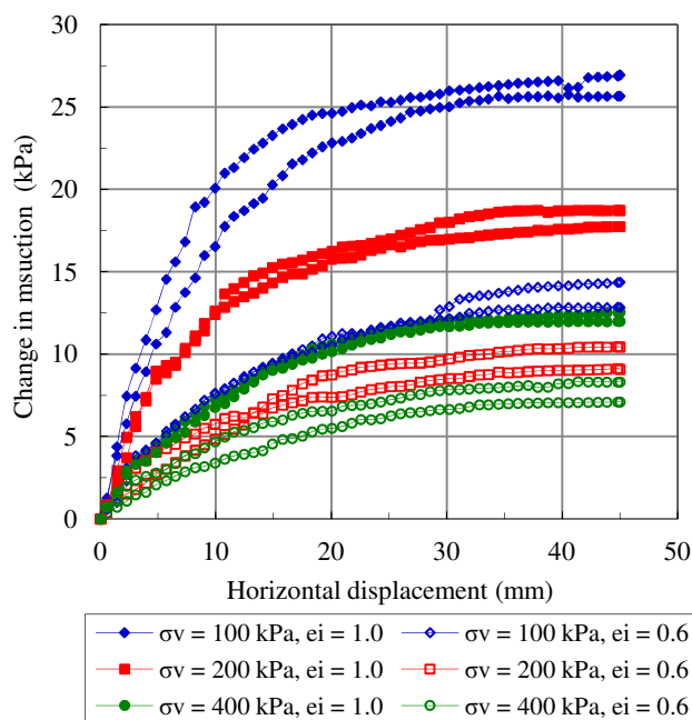
Fig. 6. Evolution of matric suction with horizontal displacement during shearing process of soil samples at e_i = 0.6 and 1.0.
