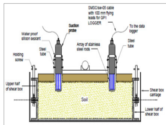
Fig. 2. Schematic drawing of modified shear cell used for soil tests at constant water content condition (not to scale).
