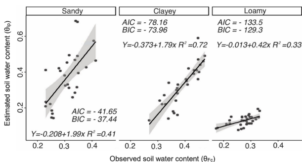
Figure 1. Correlation models between estimated water content by inflection point and water content measured at field capacity in sandy, loamy and clayey soils. R^2 : coefficient of determination; AIC: Akaike information criterion; BIC: Bayesian information criterion. The gray hatched area represents a confidence interval of 95 %.
