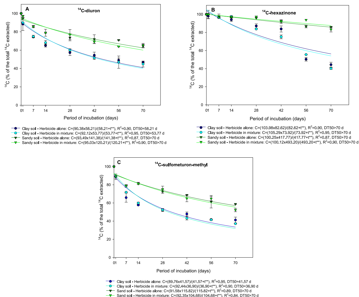
Fig. 4. Degradation of the 14 C-diuron (A), 14 C-hexazinone (B), and 14 C-sulfometuron-methyl (C) compared to the amount of each herbicide after extraction in time (extractable residue), separated by TLC plates in parental compound (%) when applied alone and in sand and clay soils, as a function of incubation time (70 d) in soil samples. The vertical bars inserted in the symbols and bars represent the standard deviation ( \pm SD) of the mean ( n = 2 ). ^{**}p < 0.01 by the F test.
