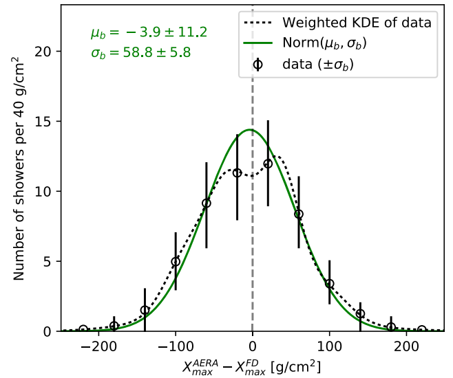
FIG. 13. Results of the comparison of X_{\max} for 53 showers measured with both FD and AERA. Plotted is the weighted KDE (black dashed curve) of the event-to-event differences in X_{\max} [sum of 53 Gaussian distributions with the individual differences as means and combined AERA and FD uncertainty \delta = (\delta_{X_{\max}^{\text{AERA}}}^2 + \delta_{X_{\max}^{\text{FD}}}^2)^{0.5} as widths]. The black markers show the spread on the KDE, evaluated at intervals of 40 \text{ g cm}^{-2} , obtained by repeatedly taking N = 53 samples from the KDE. The calculated weighted mean \mu_b and width \sigma_b of the differences are annotated in the figure (uncertainties are calculated by bootstrap resampling where we repeatedly sample 75% of events). For comparison, the Gaussian distribution corresponding to \mu_b and \sigma_b is plotted as solid green curve. Note that the combined resolution of FD and AERA ( 53.3 \pm 5.7 \text{ g cm}^{-2} , as calculated from the X_{\max} uncertainties of the 53 events) can account for the spread of the difference.
