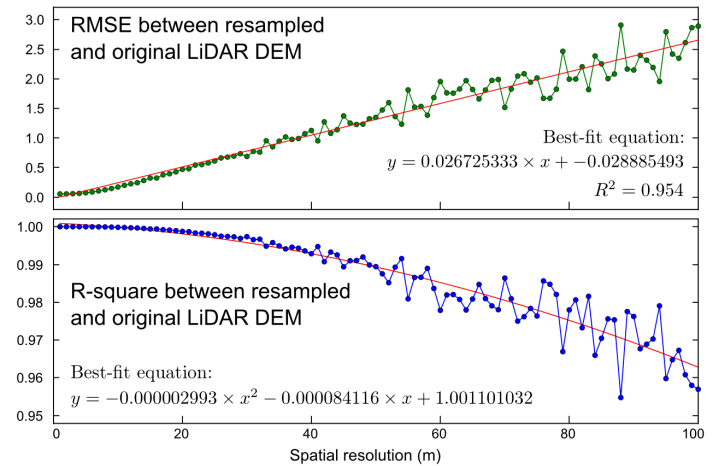
Figure 3. RSME (top) and R-squared (bottom) plots between resampled models and LiDAR data for the Garopaba dune field. Red line shows best fit of first order for RMSE values and of second order for R-squared values.
