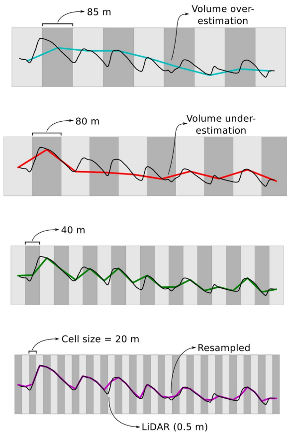
Figure 4. Topographic profiles for selected cell sizes showing effect of under- and over-estimation of volume depending on the position of the cell about the landforms.
