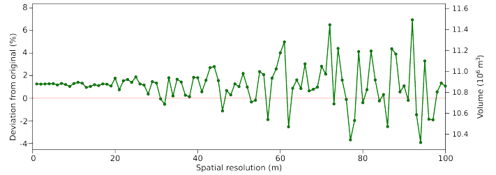
Figure 2. Volume variation with cell size and difference about the LiDAR DTM for the Garopaba dune field
