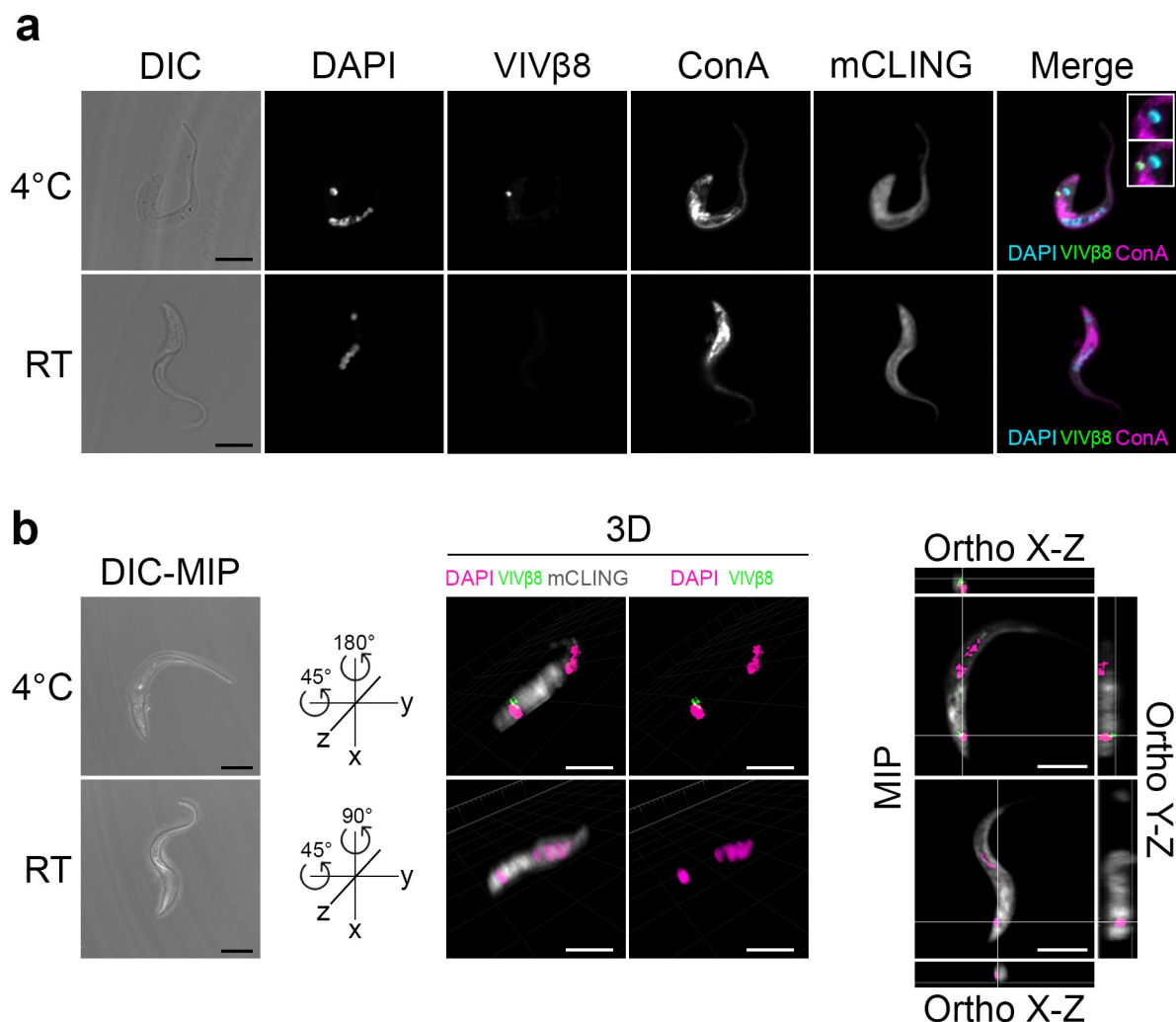
Fig 7. Live immunostaining of VIVβ8 antigen in native cells. (A) Live T. vivax bloodstream forms were immunostained either at 4°C to halt the secretory pathway or at room temperature (RT) to preserve it active. DIC; DAPI; VIVβ8 (secondary AF555-conjugated antibody); concanavalin A (ConA) FITC-conjugated lectin ER counterstain; mCLING unspecific staining and merged channels. Close-ups in merge channel show the flagellar pocket (end of ER, next to kDNA) without (top) or with (bottom) VIVβ8 green signal. Scale bars; 5 μm. (B) 3D localization of VIVβ8 in live cells. Representative cells immunostained at 4°C or RT were 3D reconstructed in DIC-maximum intensity projection (DIC-MIP, left) and rotated to equivalent positions in the space to display VIVβ8 next to the kDNA only in 4°C cells (middle). MIP fluorescence projections (right) and orthogonal views. Scale bars; 5 μm.
