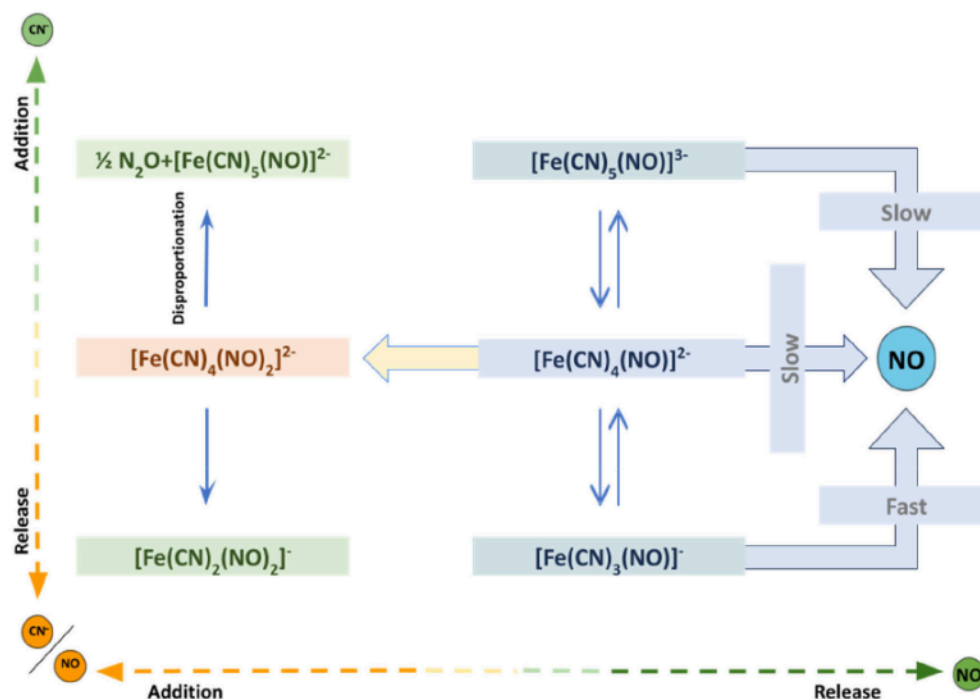
Scheme 1. Reactions between nitroprusside and thiol
