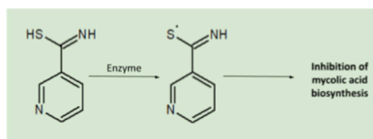
Scheme 4. Summarized action mechanism of the thionicotinamide (thiol)
