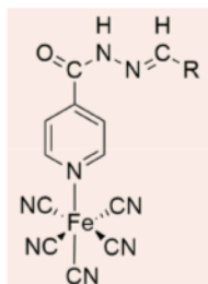
Figure 1. Structure of the derivatives of the complex [\text{Fe}^{\text{III}}(\text{CN})_5(\text{INH})]^{2-} , R = Ph (phenyl); \text{CH}_3 -4-Ph; \text{CH}_3 -O-4-Ph; F-4-Ph; Fur-2-yl
