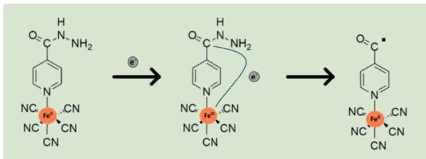
Scheme 5. Mechanism of activation of isoniazid in the complex ion [\text{Fe}^{\text{II}}(\text{CN})_5(\text{INH})]^{3-}
