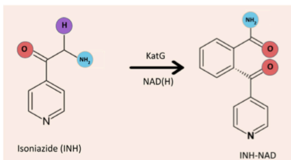
Scheme 3. The simplified mechanism of action of isoniazid
