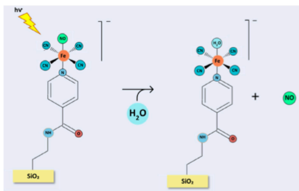
Scheme 2. NO liberation after light irradiation on the material
