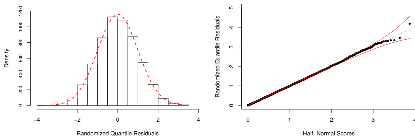
Figure 5. Frequency distribution and half-normal plot with simulated envelope for the randomized quantile residuals (RQRs).
