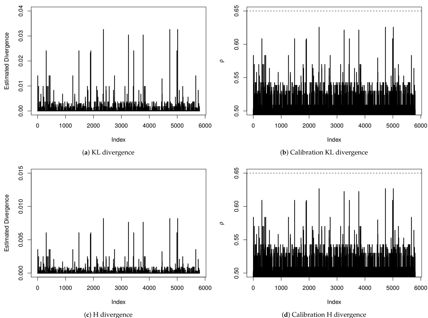
Figure 4. Sensitivity analysis for diagnosis of influential points.
