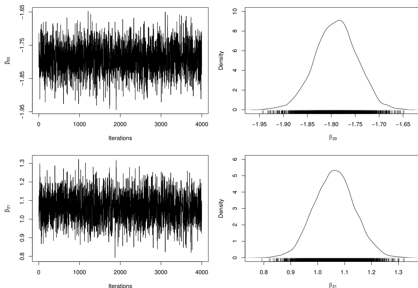
Figure 3. Trace plots and marginal posterior distributions of parameters \beta_{20} and \beta_{21} from the \mathcal{ZMPS} regression model.
