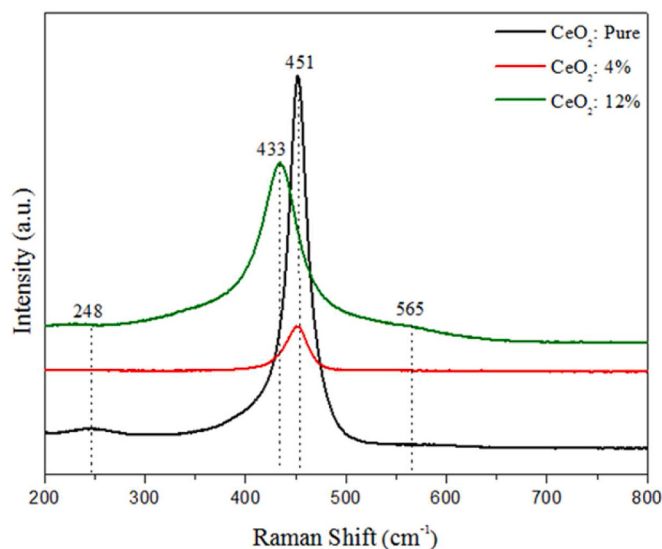
Fig. 2. Raman spectra for the pure and Co-doped \text{CeO}_2 nanopowders.
