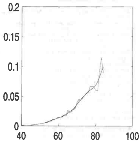
hazard rate model
