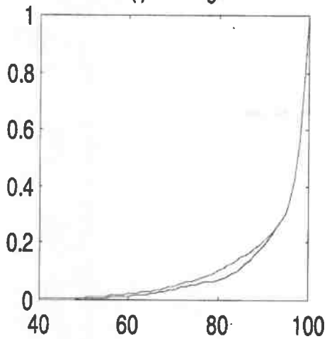
h(t) full range
