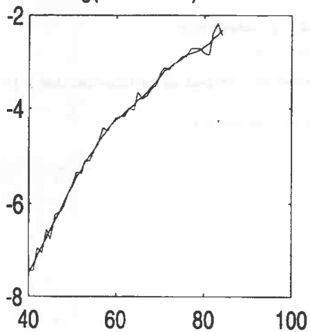
log(hazard rate) model
