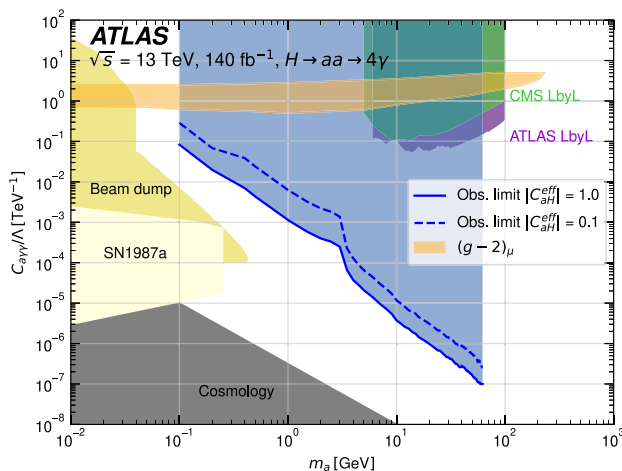
Fig. 9 Limits on the ALP mass and coupling to photons at 95% CL, assuming \mathcal{B}(a \rightarrow \gamma\gamma) = 1 , \Lambda = 1 TeV with |C_{aH}^{\text{eff}}| = 1 (solid line) and |C_{aH}^{\text{eff}}| = 0.1 (dashed line) as predicted in Ref. [19]. The shaded blue area represents the excluded region. The nearly horizontal orange shaded area indicates the region favoured by an ALP explanation for the (g-2)_\mu discrepancy [19]. Also shown are exclusion limits from the respective ATLAS [67] and CMS [68] Light-by-Light (LbyL) scattering analysis, and beam dump experiments, supernova SN1987a and cosmological observations adapted from Ref. [69]
