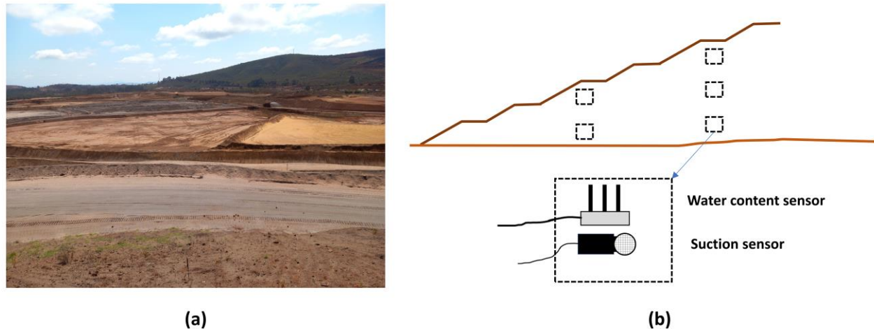
Fig 1. (a) General view of a dry stack under construction (b) schematic illustration of possible instrumentation niches.
