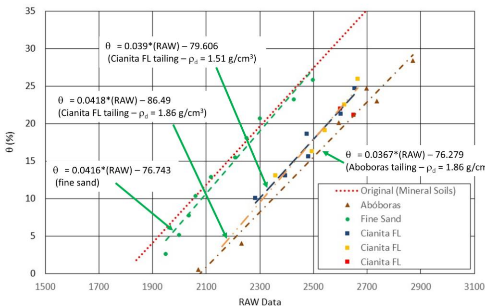
Fig. 5. Calibration data and equations for each test performed.
