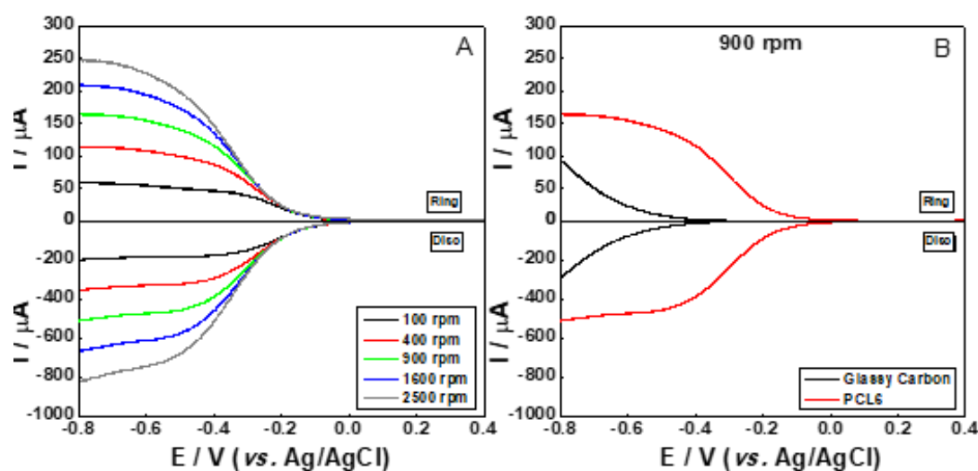
Figure 4: Steady state polarization curves for ORR using RRDE system with PCL6 at different rotations (A) along with comparison between PCL6 and GC (B). The electrolyte employed was 0.1 \text{ mol L}^{-1} \text{ K}_2\text{SO}_4 at pH 2.0 saturated with \text{O}_2 ; the scan rate was 5 \text{ mVs}^{-1} .
