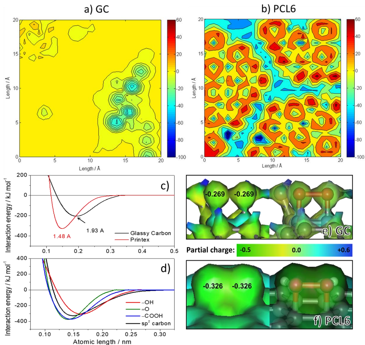
Figure 3: O 2 adsorption energy surface for (A) GC and (B) PCL6, (C) and (D) equilibrium atomic length energy curve and Mulliken partial charges along with electron density surface in the region around O 2 adsorbed on (E) GC and (F) PCL6.
