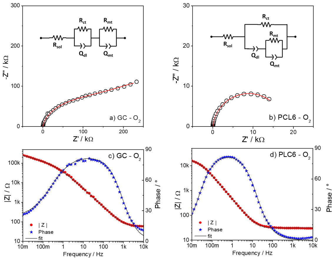
Figure 5: Nyquist and equivalent circuits used to adjust the (A) GC and (B) PLC6 data. Bode Impedance Modulus and Bode Phase for (C) GC and (D) PLC6. The electrolyte was saturated with O 2 , and the electrode was spun at 900 rpm.
