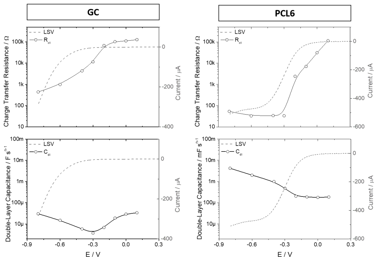
Figure 6: Impedance parameters: charge transfer resistance and double layer capacitance in relation to applied potential and LSV curve at 900 rpm.
