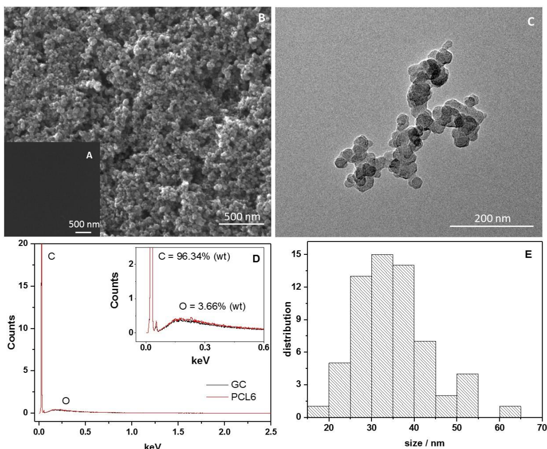
Figure 1: FEG-SEM micrographs for GC (A) and PCL6 (B) samples and the respective EDX spectra (D) for GC (black line) and PCL6 (red line). TEM analysis (C) and particle size distribution (E) for PCL6.
