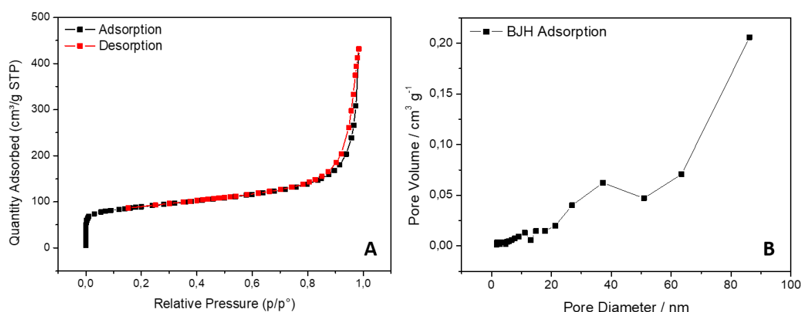
Figure 2: Brunauer-Emmett-Teller (BET) isotherm (A) and Barrett-Joyner-Halenda (BJH) pore size distribution (B) for PCL6
