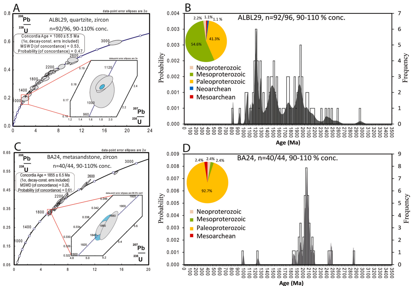
Fig. 14. U–Pb ages for detrital zircon grains from samples ALBL29 (quartzites of the Tachdamt Formation) and BA24 (metasandstone of the Bleida Formation) of the lower Anti-Atlas Supergroup. (A) and (C) are concordia diagrams; (B) and (D) are combined binned frequency and probability density plots of detrital zircon grains. Abbreviations: Conc.-Concordance; Decay-const. errors- Decay-constant errors.
