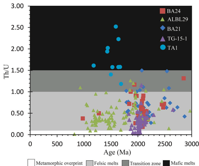
Fig. 8. Th/U ratios versus concordant U-Pb ages of igneous and detrital zircon grains of the lower Anti-Atlas Supergroup.
