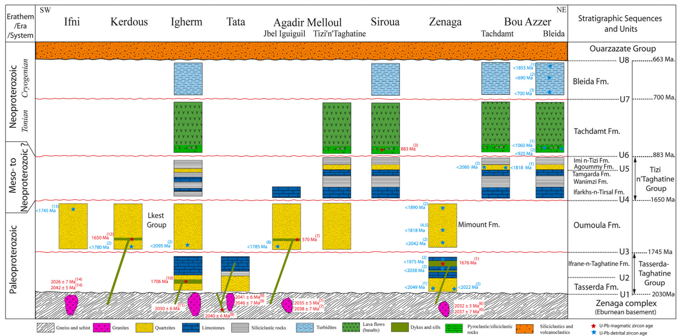
Fig. 18. A tentative correlation scheme of the lower Anti-Atlas Supergroup and its stratigraphic equivalents in the Anti-Atlas inliers. U1 to U8 are unconformities. U–Pb geochronology data are from (1) this study, (2) Letsch (2018), (3) Youbi et al. (2018) and Bouougri et al. (2020) Bouougri et al. (2020), (4) Abati et al. (2010), (5) Walsh et al. (2012), (6) Thomas et al. (2002), (7) Soulaïmani et al. (2013), Hafid et al. (2013), Blein et al. (2014b), (8) Soulaïmani et al. (2019), (9) Walsh et al. (2002), (10) Ikenne et al. (2017), (11) Aït Malek et al. (1998), (12) Youbi et al. (2019), (13) Benziane et al. (2016), and (14) Schulte et al. (2016).
