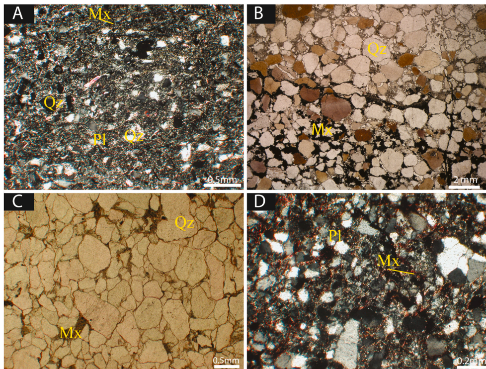
Fig. 12. Thin section photomicrographs of the sedimentary samples. (A) Metasiltstones of the Tasserda Formation: sample TG-15-1; purple, coarse-grained and quartz-rich met-siltstone with quartz (Qz) and feldspar (Pl) embedded in a sericite-rich matrix (Mx); crossed nicols. (B) Quartzites of the Agoumy Formation: sample BA21, with quartz grains that are mostly subrounded. (C) Quartzites of the Tachdamt Formation: sample ALBL29, with a mineral assemblage comprised mainly of quartz (Qz) associated to a small amount of feldspars (Pl) with a matrix (Mx) of silt-sized quartz and mica minerals. (D) Metasandstone of the Bleida Formation: sample BA24, fine-grained, moderately sorted metasandstone with quartz (Qz), plagioclase (Pl), and lithic fragments in mica matrix (Mx). (For interpretation of the references to colour in this figure legend, the reader is referred to the Web version of this article.)
