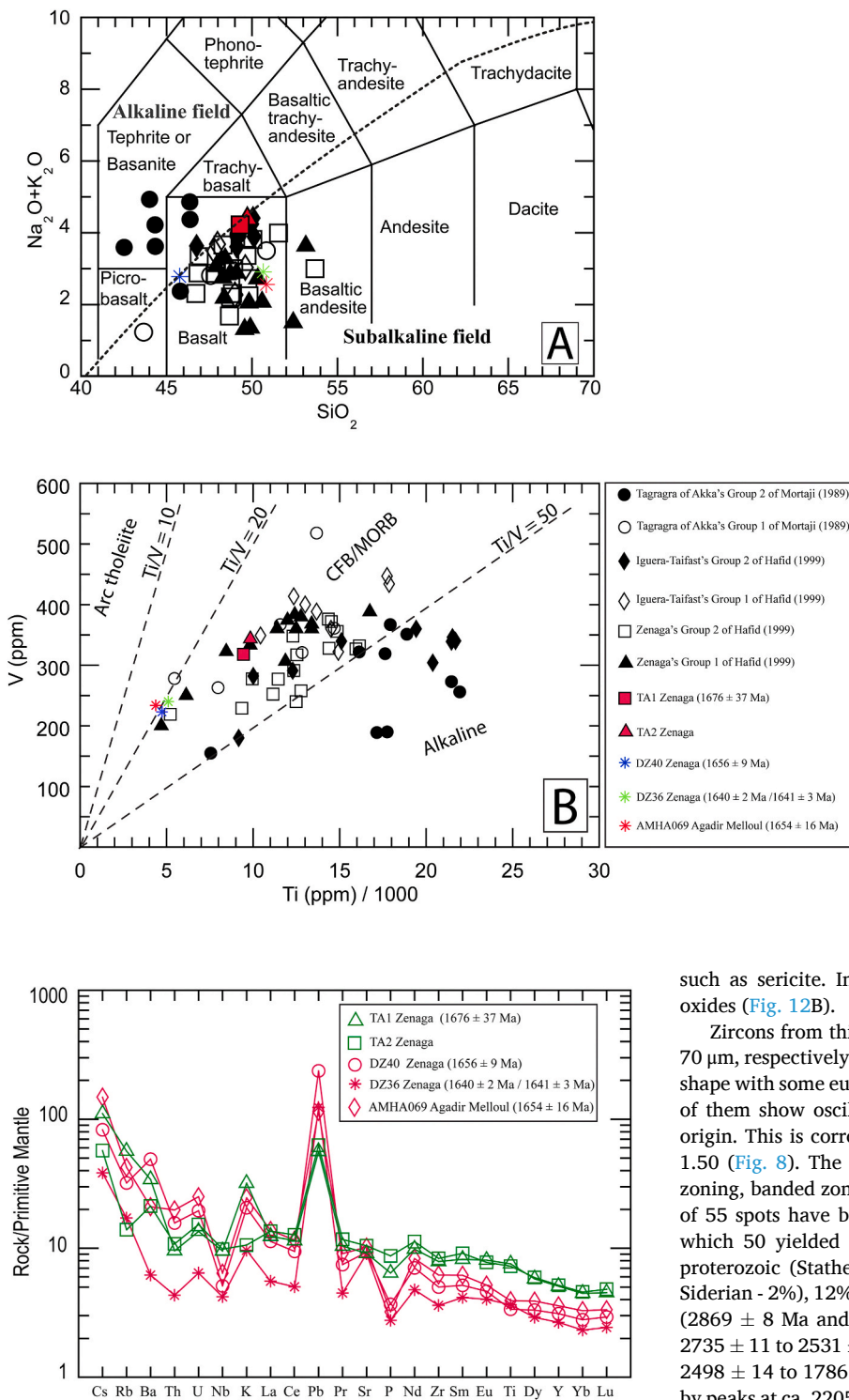
Fig. 11. Primitive mantle-normalized trace element 'spidergram' for the dated mafic sill and dykes of the Zenaga and Agadir Melloul inliers. Primitive mantle values used for normalization are from Sun and McDonough (1989) .
