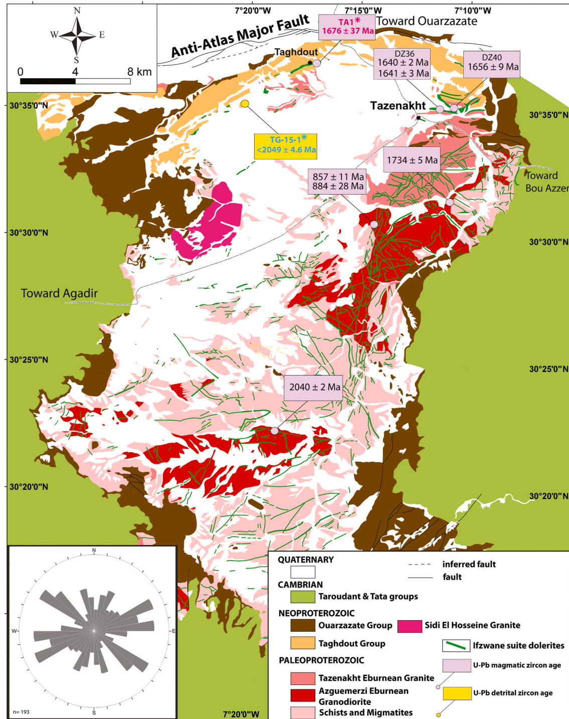
Fig. 4. Geology of the Zenaga Inlier (modified after Choubert, 1963; Ennih and Liégeois, 2001; Thomas et al., 2002; Kouyaté et al., 2013; Youbi et al., 2013). The Taghdout Group corresponds to the lower Anti-Atlas Supergroup (Thomas et al., 2004). Inset shows a rose diagram that summarizes mafic dyke trends measured from the map and Google Earth; n is the number of measurements. The U-Pb ages obtained in this study are indicated with asterisks; other age constraints are from literature (Kouyaté et al., 2013; Youbi et al., 2013).
