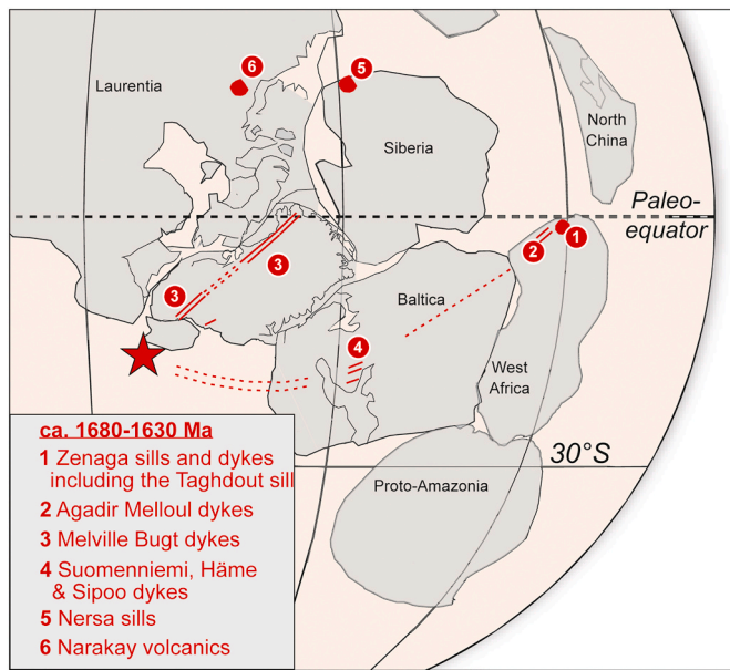
Fig. 15. Paleomagnetically and geologically informed reconstruction of WAC, Amazonia, and Baltica cratons (SAMBA connection) along with Laurentia and Siberia in the core of the Nuna supercontinent (modified after Evans and Mitchell, 2011 ); additional ca. 1640–1680 Ma dyke swarms include the 1641 ± 8 Ma Nersa sill complex of Southern Siberia (U–Pb baddeleyite TIMS age; Metelkin et al., 2011 ; Ernst et al., 2016 ), 1635.0 ± 2.7 to 1622.1 ± 3.2 Ma Melville Bugt dykes of western Greenland (U–Pb baddeleyite TIMS age; Halls et al., 2011 ; Klausen and Nilsson, 2019 ), 1663 ± 8 Ma bimodal Narakay Volcanic Complex of Canada (U–Pb zircon TIMS age; Bowring and Ross, 1985 ), and 1642 ± 2 Ma dyke swarms of Häme, Sipoo, and Suomenniemi of the Fennoscandian Shield in southeast Finland (U–Pb ID-TIMS baddeleyite age; Vaasjoki et al., 1991 ; Salminen et al., 2017 ). Star locates mantle plume centre, proposed for the Melville Bugt swarm by Klausen and Nilsson (2019) .
