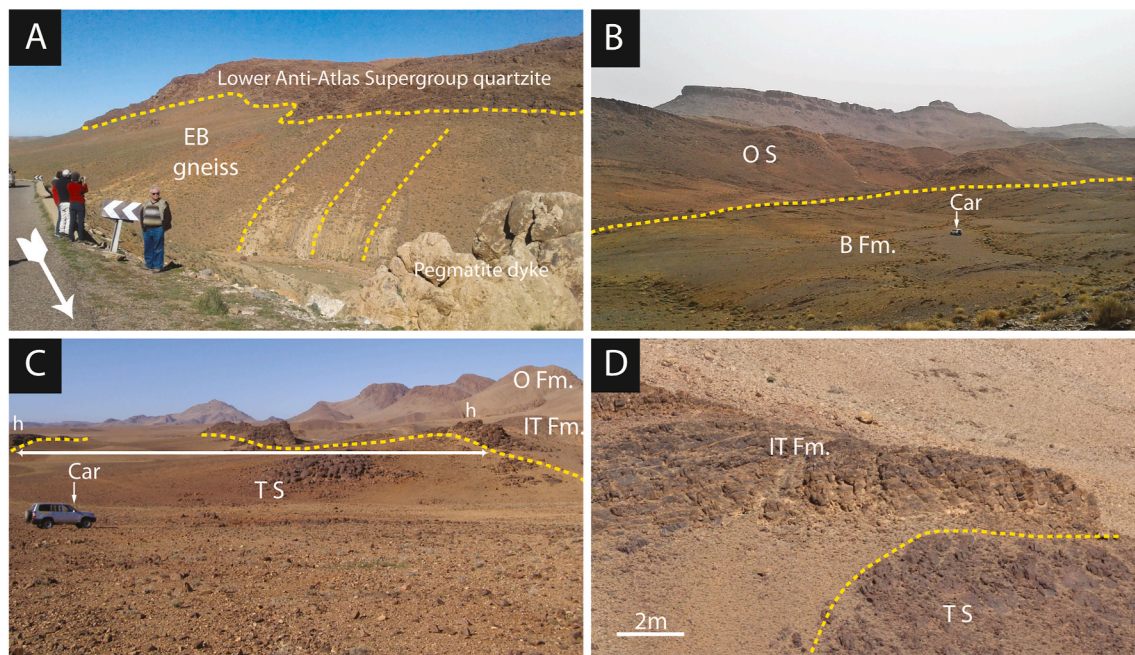
Fig. 6. (A) General view of the unconformity between the Eburnean basement and the overlying quartzites of Oumoula Formation (O Fm.) of the lower Anti-Atlas Supergroup at Tizi n'Taghatine locality. The Eburnean basement (EB: gneiss and schists) is crosscut by pegmatite dyke. The arrow indicates the road from Taliwine to Tazenakht. Geologists are Fida Medina, Maria Giuditta Fellin, Claudio Faccenna, and Riccardo Lanari; (B) View of the unconformity between the schists of the Bleida Formation (B Fm.) and the overlying volcanic rocks of the Ouazazate Supergroup (OS); (C) View of the Taghdout sill (TS) crosscutting the mixed siliciclastic-carbonate succession of the Ifrane-n-Taghatine Formation (IT Fm.) in the Zenaga Inlier near the Taghdout Town. Note hornfels (h) at the baked margin of the sill. The Ifrane-n-Taghatine Formation is overlain by thick quartzites of Oumoula Formation (O Fm.); and (D) Detailed view of the upper contact between the Taghdout dolerite sill (TS) and limestones of the Ifrane-n-Taghatine Formation (IT Fm.) transformed into hornfels.
