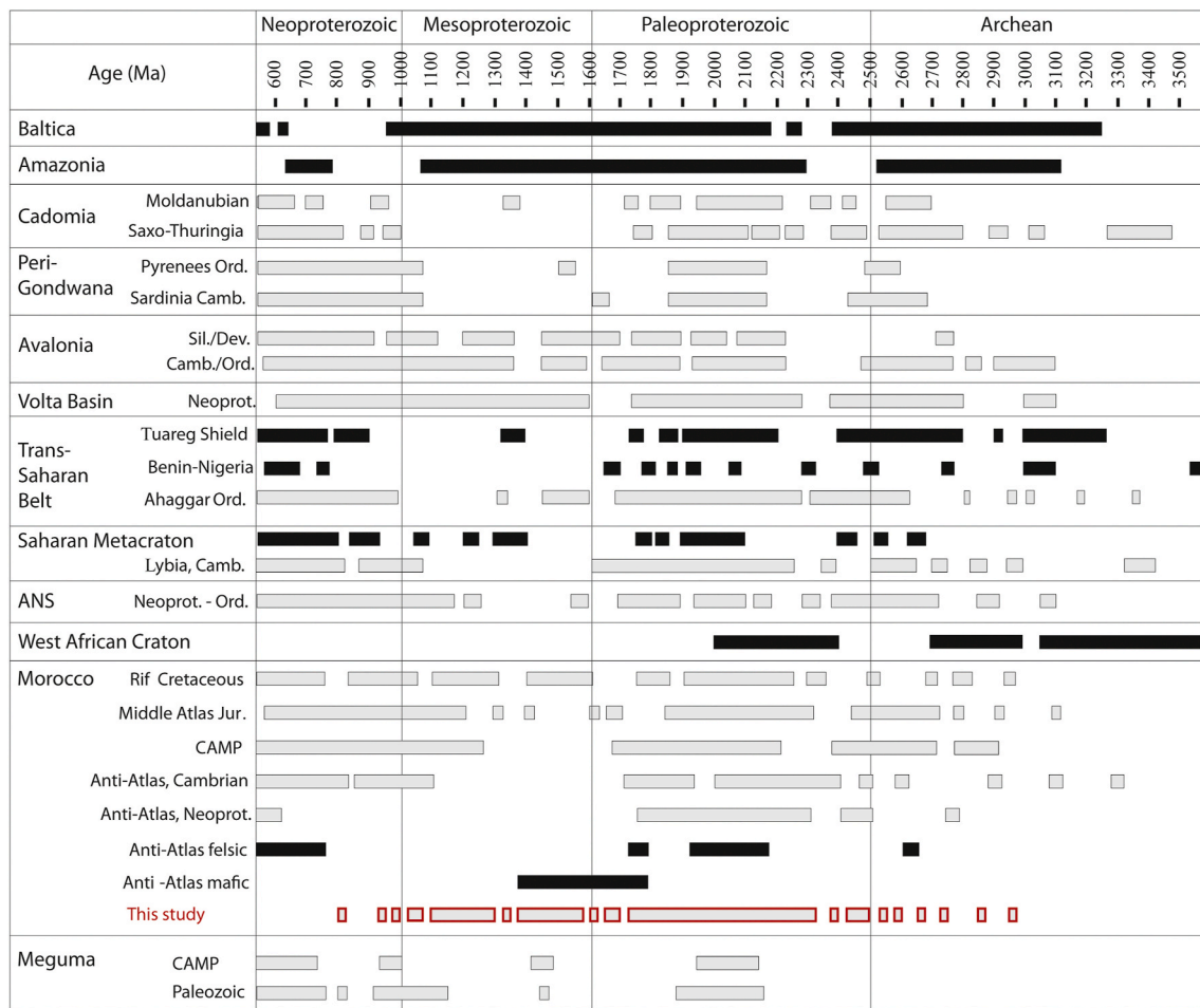
Fig. 17. Distribution of U–Pb ages for detrital zircon grains analyzed in this study from the lower Anti-Atlas Supergroup in the Zenaga and Bou Azzer El Graara inliers (all grouped together) and potential sources compiled from the literature. Grey stripes: detrital zircons; black stripes: zircons from magmatic rocks. Detrital zircon data sources: Pyrenees (Margalef et al., 2016); Lybia (Altumi et al., 2013); Algeria, Ahaggar (Linnemann et al., 2011); Meguma, Ganderia, and Avalonia detrital zircons (Fyffe et al., 2009; Gärtner et al., 2016; Henderson et al., 2016; Murphy et al., 2004a, 2004b; Waldron et al., 2009 and references therein); Anti-Atlas and Sardinia Cambrian (Avigad et al., 2012); Anti-Atlas Neoproterozoic (Abati et al., 2010; Karaoui et al., 2015). Anti-Atlas mafic rocks (Youbi et al., 2013 and references therein). Modified after Linnemann et al. (2011), Pratt et al. (2015), and Marzoli et al. (2017), and references therein. Abbreviations: ANS = Arabian–Nubian Shield; CAMP=Central Atlantic Magmatic Province; Camb.-Cambrian; Dev.- Devonian; Jur., Jurassic; Neoprot.- Neoproterozoic; Ord.- Ordovician; Sil.-Silurian.
