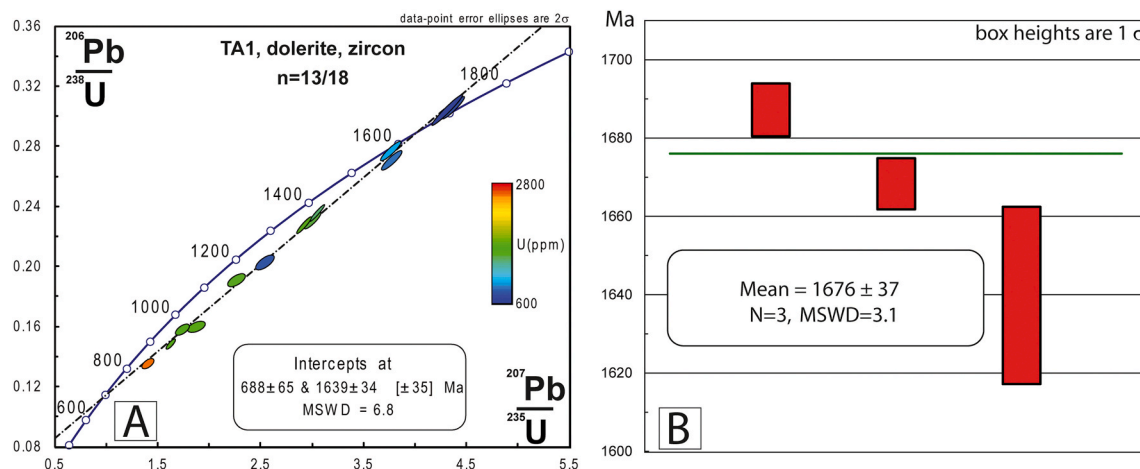
Fig. 9. Zircon U-Pb SHRIMP geochronology: (A) Wetherill concordia plots of U-Pb zircon data for the Taghadout sill (sample TA) of the Zenaga Inlier. (B) Weighted mean average ^{207}\text{Pb}/^{206}\text{Pb} age of analysis with low Th and U concentrations (spots 2.1, 7.1, and 13.1).
