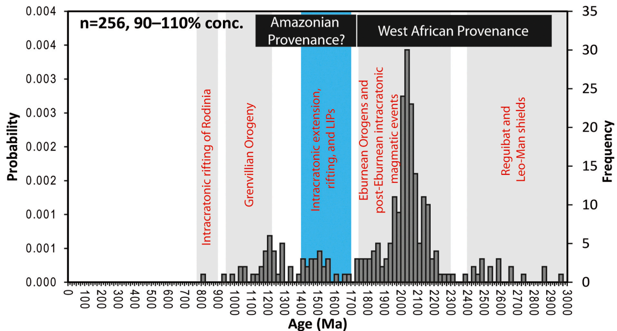
Fig. 16. Age compilation for detrital zircon grains from four samples collected from the lower Anti-Atlas Supergroup in the Zenaga and Bou Azzer El Graara inliers. Ages older than 1.7 Ga indicate the West African provenance (modified from Linnemann et al., 2010 and Abubaker et al., 2017). See the text for more explanation. Abbreviations: Conc.-Concordance.
