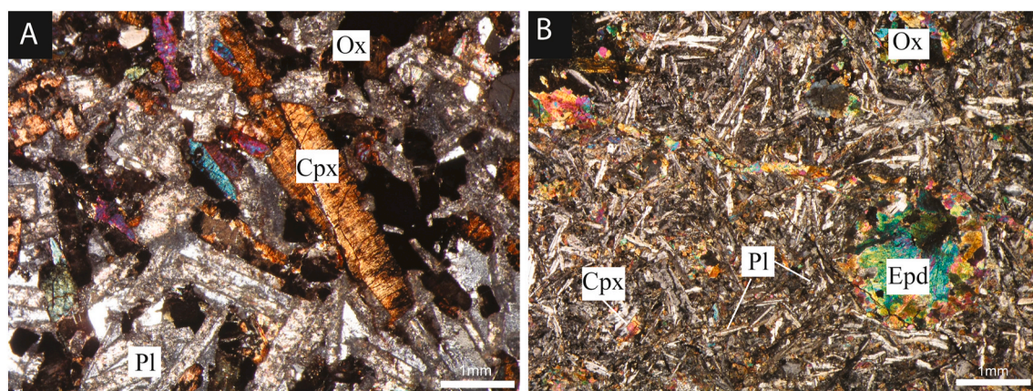
Fig. 7. Thin-section photomicrographs of the Great Taghdout sill. (A) coarse-grained dolerite in the centre of the sill with plagioclase (Pl) and clinopyroxene (Cpx) minerals and oxides (Ox), crossed nicols; (B) fine-grained, microlitic porphyric texture at the border of the sill with microlites (tiny crystals) of plagioclase (Pl) and clinopyroxene (Cpx) minerals and oxides (Ox). Epidote (Ep) is filling vesicles; crossed nicols.
