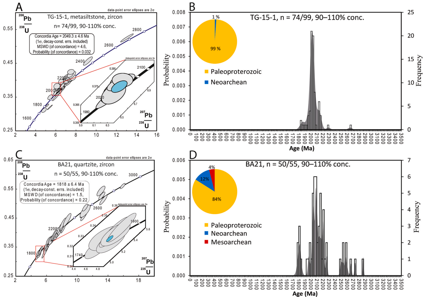
Fig. 13. U–Pb ages for detrital zircon grains from samples TG-15-1 (metasiltstones of the Tasserda Formation) and BA21 (quartzites of the Agoumy Formation) of the lower Anti-Atlas Supergroup. (A) and (C) are concordia diagrams; (B) and (D) are combined binned frequency and probability density plots of detrital zircon grains. Abbreviations: Conc.-Concordance; Decay-const. errs.- Decay-constant errors.
