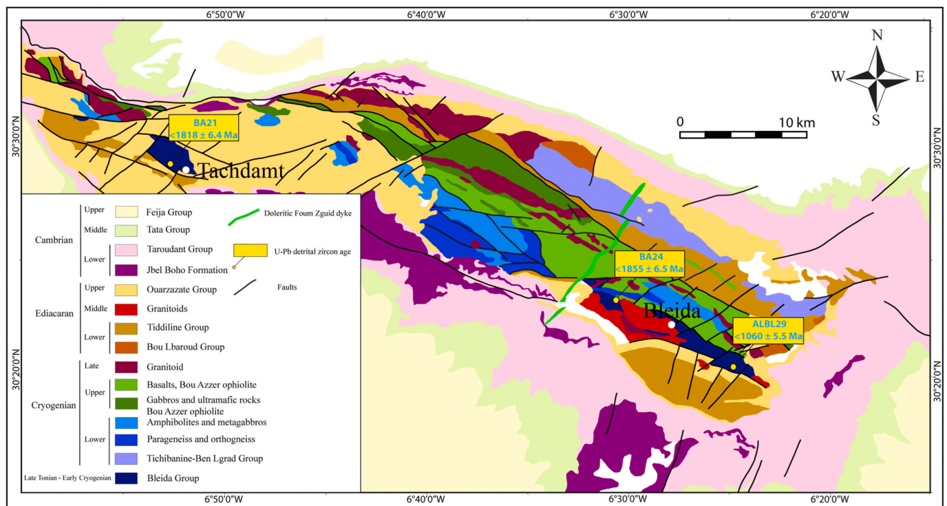
Fig. 5. Simplified geological map of the Bou Azer-El Graara Inlier showing the main lithotectonic units. The localities (Tachdamt and Bleida) mentioned in the text are indicated, as well as the location of samples used for U–Pb detrital geochronology (after Blein et al., 2014a). The Bleida Group corresponds to the lower Anti-Atlas Supergroup (Blein et al., 2014a).
