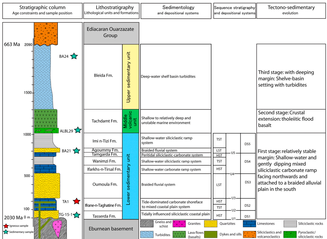
Fig. 3. Lithostratigraphic subdivision, sequence stratigraphy, and paleogeographic data for the lower Anti-Atlas Supergroup (modified after Bouougri and Saquaque, 2004). We use the name of the Ifrane-n-Taghatine Formation instead of the Taghdout Formation to avoid confusion with the widely used name of the group - "the Taghdout Group" in the Zenaga Inlier. Abbreviations: systems tracts consist of (LST) lowstand system tracts, (TST) transgressive system tracts, and (HST) highstand system tracts. U1 to U5 are unconformities. DS1 to DS5 are depositional systems.
