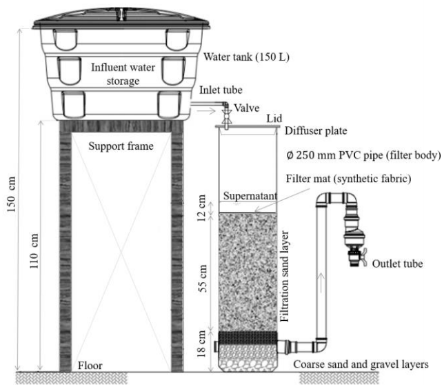
Figure 1. HSSF researched in continuous flow.
