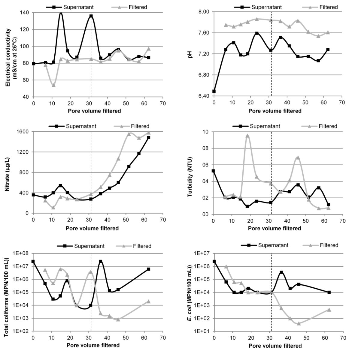
Figure 3. Filter performance adding 0.25 g/day of fish food using highly contaminated influent water during the second phase (water temperature = 24.5±0.5 °C) for twelve sequential days of operation. Vertical dashed lines indicate when the influent water was renewed.
