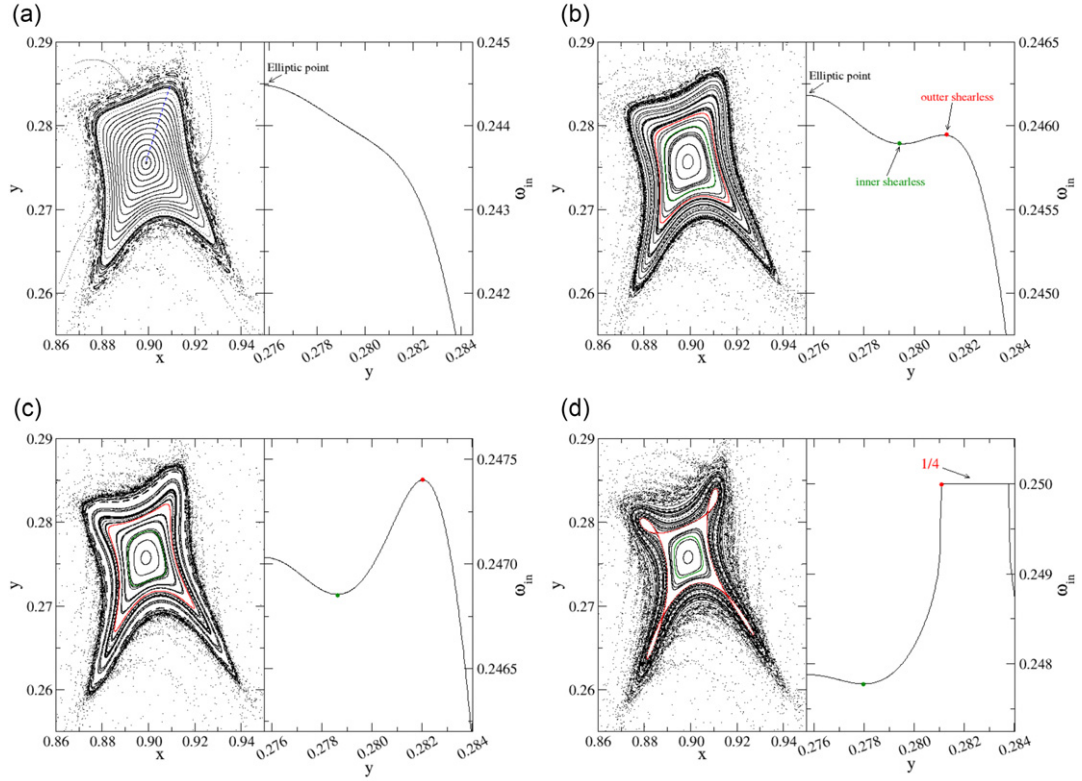
Figure 5. The quadrupling bifurcation in the Ullmann map. (a) \epsilon = 0.185 ; (b) \epsilon = 0.187 ; (c) \epsilon = 0.188 and (d) \epsilon = 0.189 . Note that the onset of two s-shearless tori arose for some value of \epsilon between (a) and (b).
