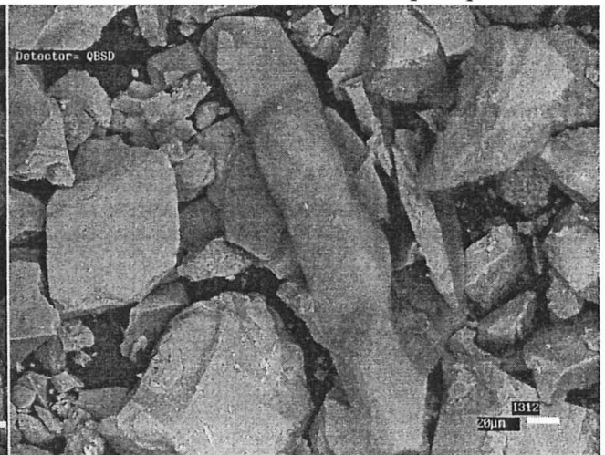
7- General aspect of apatite in the final flotation concentrate
