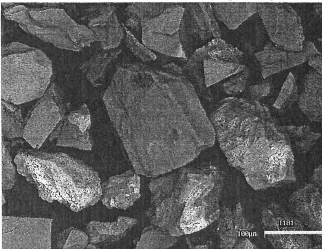
6- General aspect of apatite in the feed of the coarse friable flotation circuit
