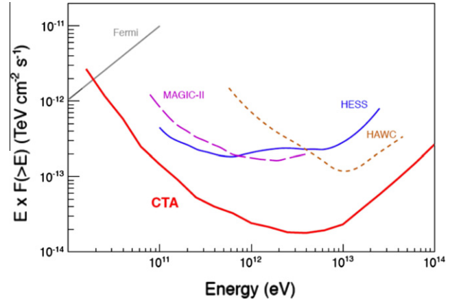
Fig. 8. Integral sensitivity for CTA from MC simulations, together with the sensitivities in comparable conditions (50 h for IACTs, 1 year for Fermi-LAT and HAWC) for some gamma-ray observatories.
