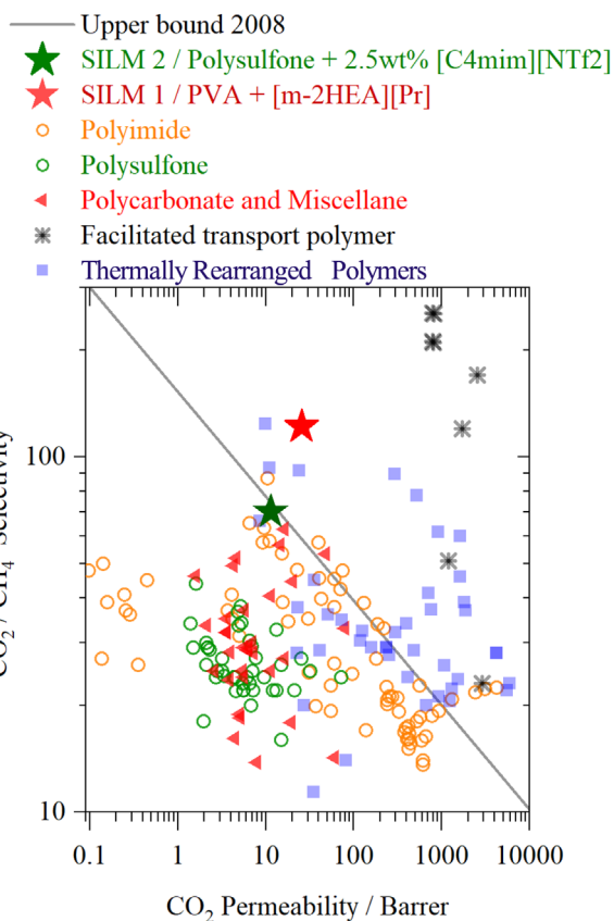
Figure 18. Permeability/selectivity trade-off for polymeric membranes tuned either by the polymer chemical structure or by the IL-facilitated transport. Data collected from elsewhere. 247,264 SILM 1 refers to data from Alcantara et al., 266 and SILM 2 refers to data from Alkhouzaam et al. 265
