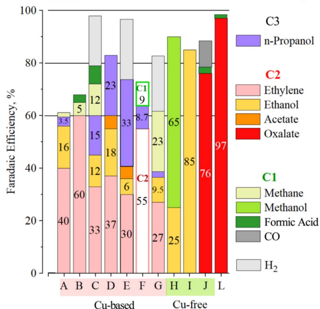
Figure 22. Faradaic efficiency of CO 2 electroreduction on copper-based electrocatalysts (references A–G), copper-free electrocatalysts (references H–J), or a catalyst-free platform (L) based on a range spectrum of the final products (C3, n-propanol; C2, ethylene, ethanol, acetate, and oxalate; C1, methane, methanol, formic acid, and carbon monoxide; and hydrogen). References D and E tested the carbon monoxide reduction reaction. Reprinted with permission from (A. Mota-Lima, J. Phys. Chem. C , 124 , 10907, 2020). 327 Copyright (2021) American Chemical Society.
