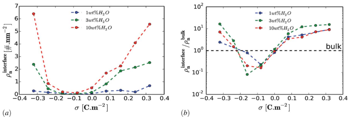
Figure 19. Electrodesorption of water on graphene from water-containing relin (chl: urea 1:2) contacting a graphene interface. The averaged (a) and normalized (b) number density of adsorbed water in the interfacial region as a function of surface charge density. The number of residual water molecules in bulk Relin is 1 wt%, 3 wt%, and 10 wt%. The interfacial region is taken to be 3.5 Å from the graphene surface. Reproduced from “Mamme et al. Nanoscale Advances , 1, 2847, 2019” 288 —Published by The Royal Society of Chemistry.
