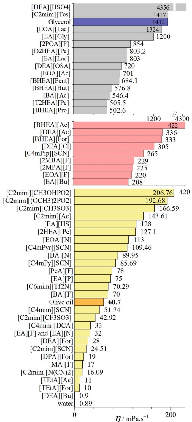
Figure 3. Dynamic viscosities ( \nu ) of 48 ionic liquids measured at T = 298.15 K and P = 1 bar by different authors as Zhao et al. 2008, 39 Chennuri & Gardas 2016, 36 Iglesias et al. 2010, 38 Widgren & Magee 2007, 31 Greaves et al. 2006, 41 Xu 2013, 35 Domanska & Królikowska 2012, 37 Alcantara et al. 2018 40 and Freire 2011. 34 The viscosities of water, olive oil and glycerol are also shown for getting IL-viscosities into perspective.
