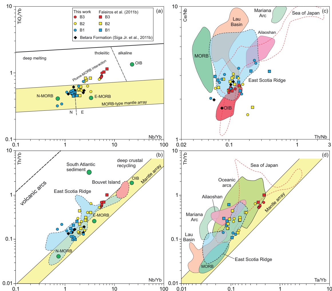
Fig. 12. Petrogenetic and tectonic discriminant diagrams with geochemical data of Votuverava metabasites. (a) Nb/Yb versus \text{TiO}_2/\text{Yb} plot (after Pearce, 2008), (b) Nb/Yb versus Th/Yb plot (after Pearce, 2008), (c) Th/Nb versus Ce/Nb plot (modified from Sandeman et al., 2006), (d) Ta/Yb versus Th/Yb plot (after Pearce, 1982). Data fields: East Scotia Ridge, Bouvet Island and South Atlantic sediments (Leat et al., 2000; Fretzdorff et al., 2002); Sea of Japan (Poulet et al., 1994); Mariana Arc (Elliott et al., 1997); MORB and OIB (Pearce, 1982); Lau Basin (Pearce et al., 1994); Ailaoshan Tectonic Zone (Fan et al., 2010).
