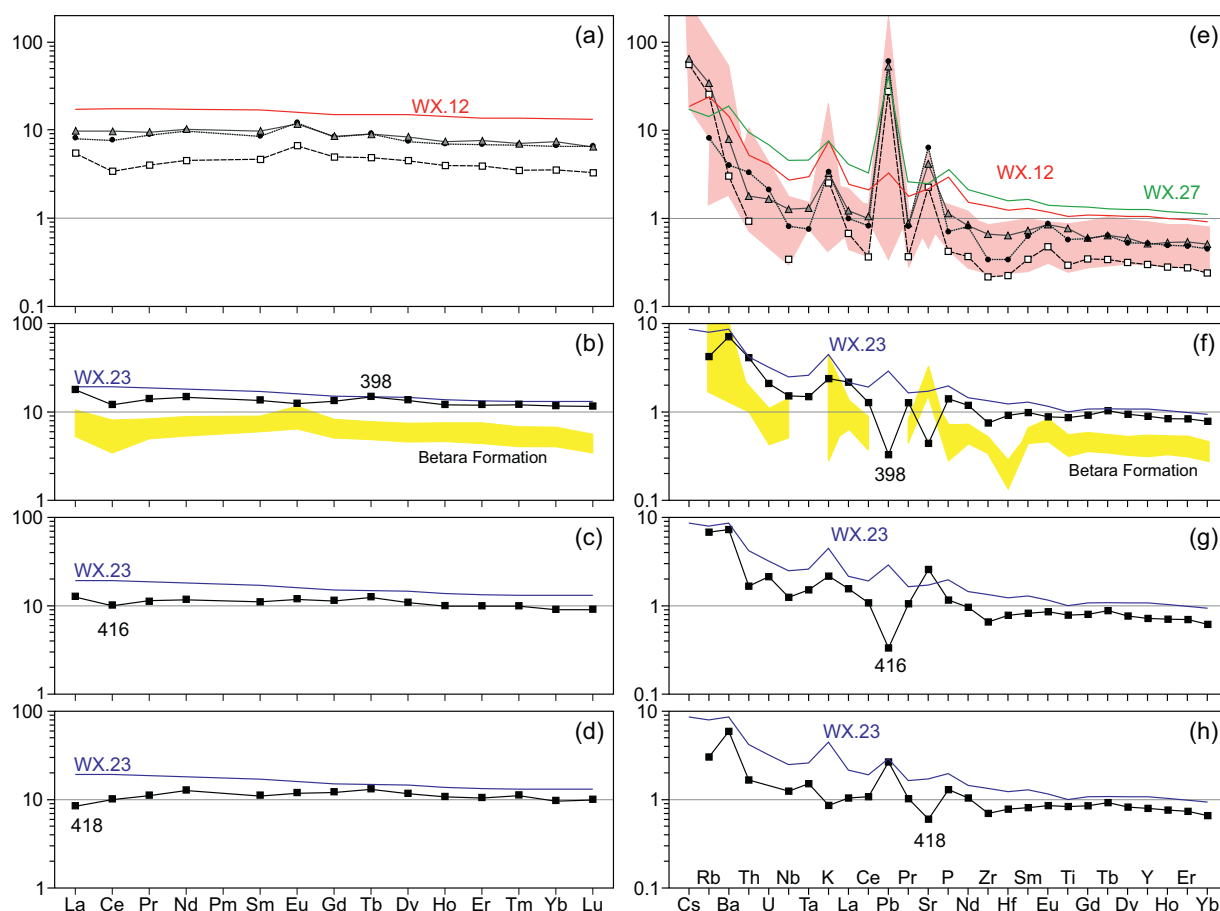
Fig. 4. Rare earth element (a–d) and incompatible element (e–h) spidergrams of the B1 group Votuverava metabasites. The colored field in (e) is the compositional range for all B1 samples. Data for the Betara Formation metabasites after Siga et al. (2011b). Samples WX.12, WX.23 and WX.27 are basalts from the East Scotia Ridge back-arc basin (Leat et al., 2000) for comparison. Normalization values from Sun and McDonough (1989) for MORB and Boynton (1984) for chondrite. (For interpretation of the references to color in this figure legend, the reader is referred to the web version of this article.)
