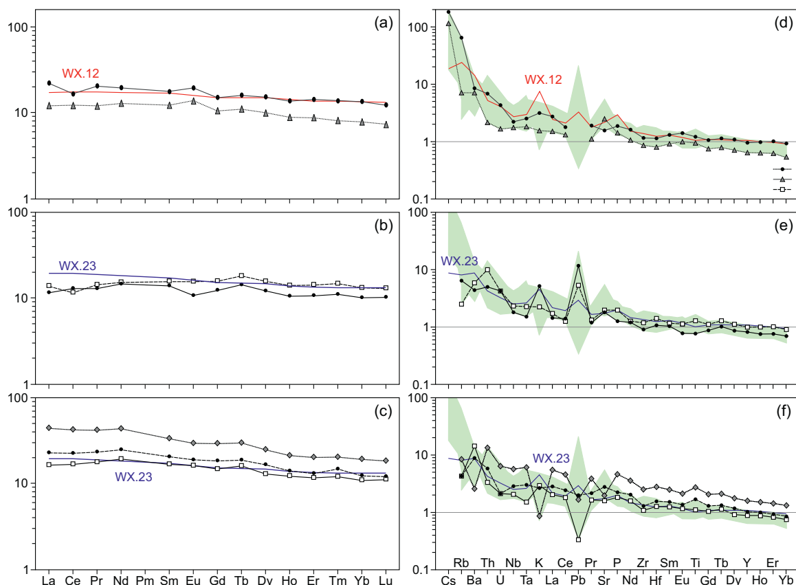
Fig. 5. Rare earth element (a–c) and incompatible element (d–f) spidergrams of the B2 group Votuverava metabasites. The colored field in (d–f) is the compositional range for all B2 samples. Samples WX.12 and WX.23 are basalts from the East Scotia Ridge back-arc basin (Leat et al., 2000) for comparison. Normalization values from Sun and McDonough (1989) for MORB and Boynton (1984) for chondrite. (For interpretation of the references to color in this figure legend, the reader is referred to the web version of this article.)
