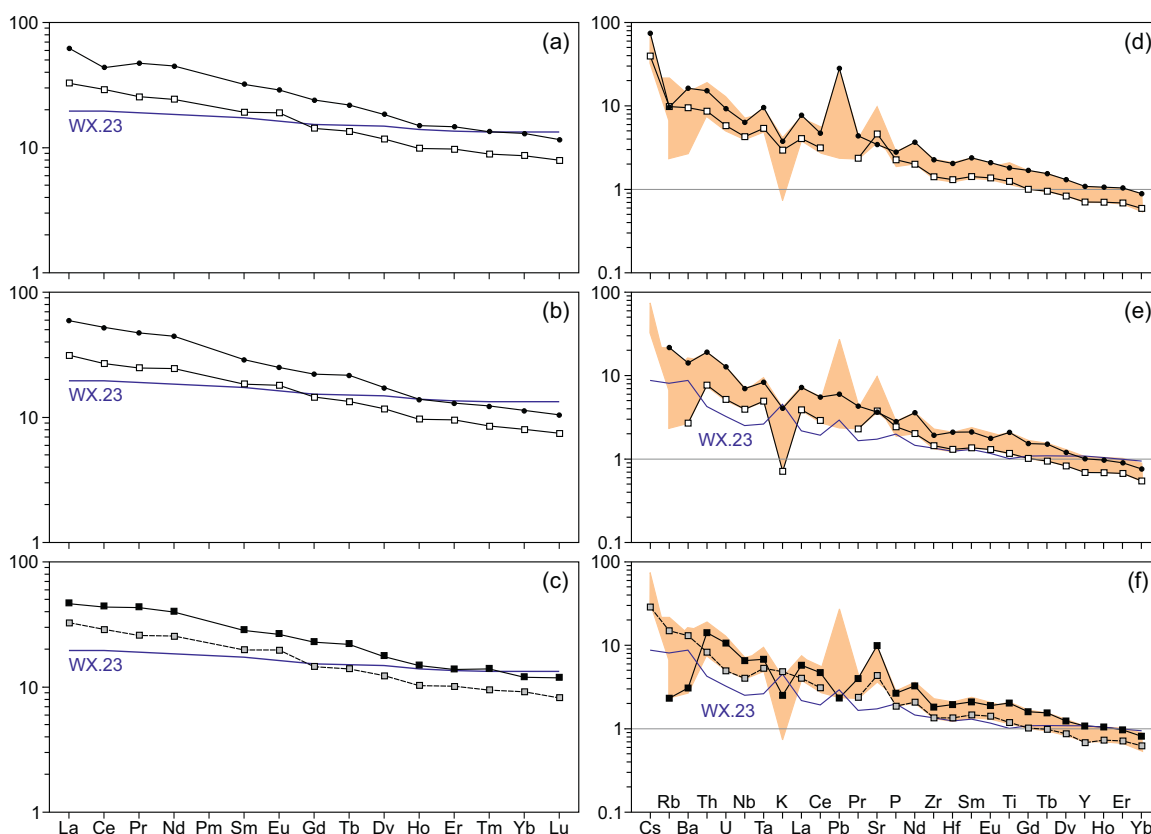
Fig. 6. Rare earth element (a–c) and incompatible element (d–f) spidergrams of the B3 group Votuverava metabasites. The colored field in (d–f) is the compositional range for all B3 samples. Sample WX.23 is a basalt from the East Scotia Ridge back-arc basin (Leat et al., 2000) for comparison. Normalization values from Sun and McDonough (1989) for MORB and Boynton (1984) for chondrite. (For interpretation of the references to color in this figure legend, the reader is referred to the web version of this article.)
