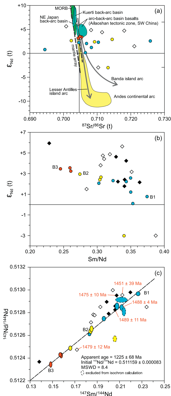
Fig. 10. Plot of initial ^{87}Sr/^{86}Sr(t) versus \epsilon_{Nd}(t) ( t = 1480 Ma). (a) Data fields and trends: MORB and mantle array (Winter, 2010), back-arc basin basalts (Shuto et al., 2006; Jian et al., 2008, 2009a,b; Fan et al., 2010), island arc and continental arc volcanics (McCulloch et al., 1994; Winter, 2010). (b) Plot of Sm/Nd versus \epsilon_{Nd}(t) . (c) Sm/Nd isochron diagram of Votuverava metabasites with error ellipses stated at the 2\sigma level. Also shown are the available zircon U–Pb age data. Circles and ellipses are data from this work. Diamonds are data compiled from Siga et al. (2011a) (white) and Siga et al. (2011b) (black).
