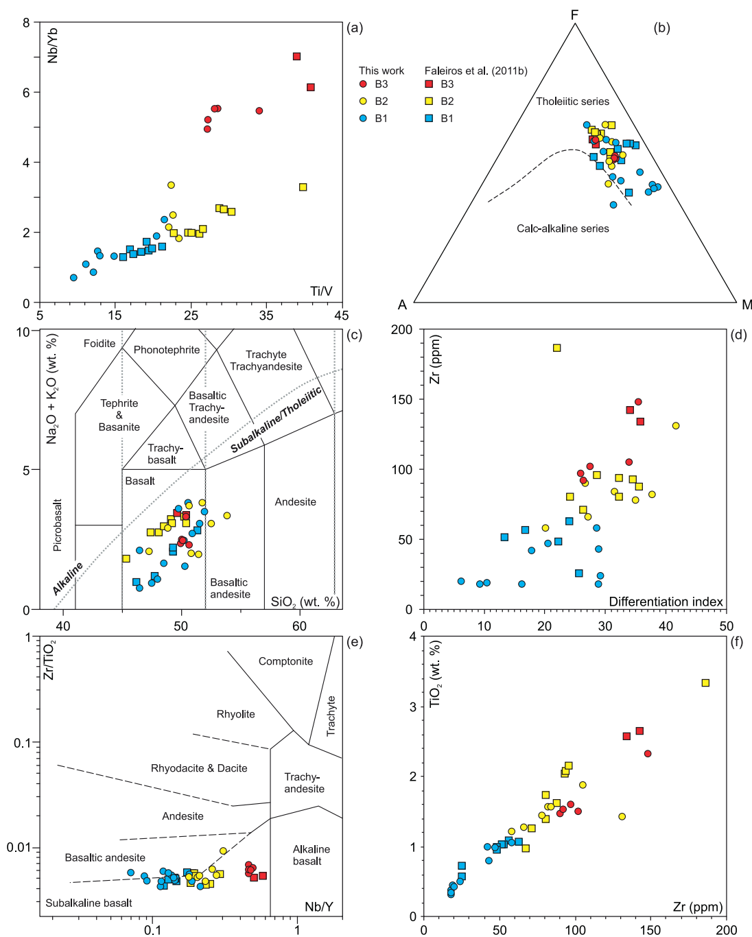
Fig. 3. Classification and petrogenetic diagrams with geochemical data of Votuverava metabasites. (a) Ti/V versus Nb/Yb plot, (b) AFM diagram after Irvine and Baragar (1971), (c) SiO 2 versus total alkalis plot after Le Bas et al. (1986), (d) differentiation index (normative quartz + albite + orthoclase) versus Zr plot, (e) Nb/Y versus Zr/TiO 2 plot after Winchester and Floyd (1977), and (f) Zr versus TiO 2 plot.
