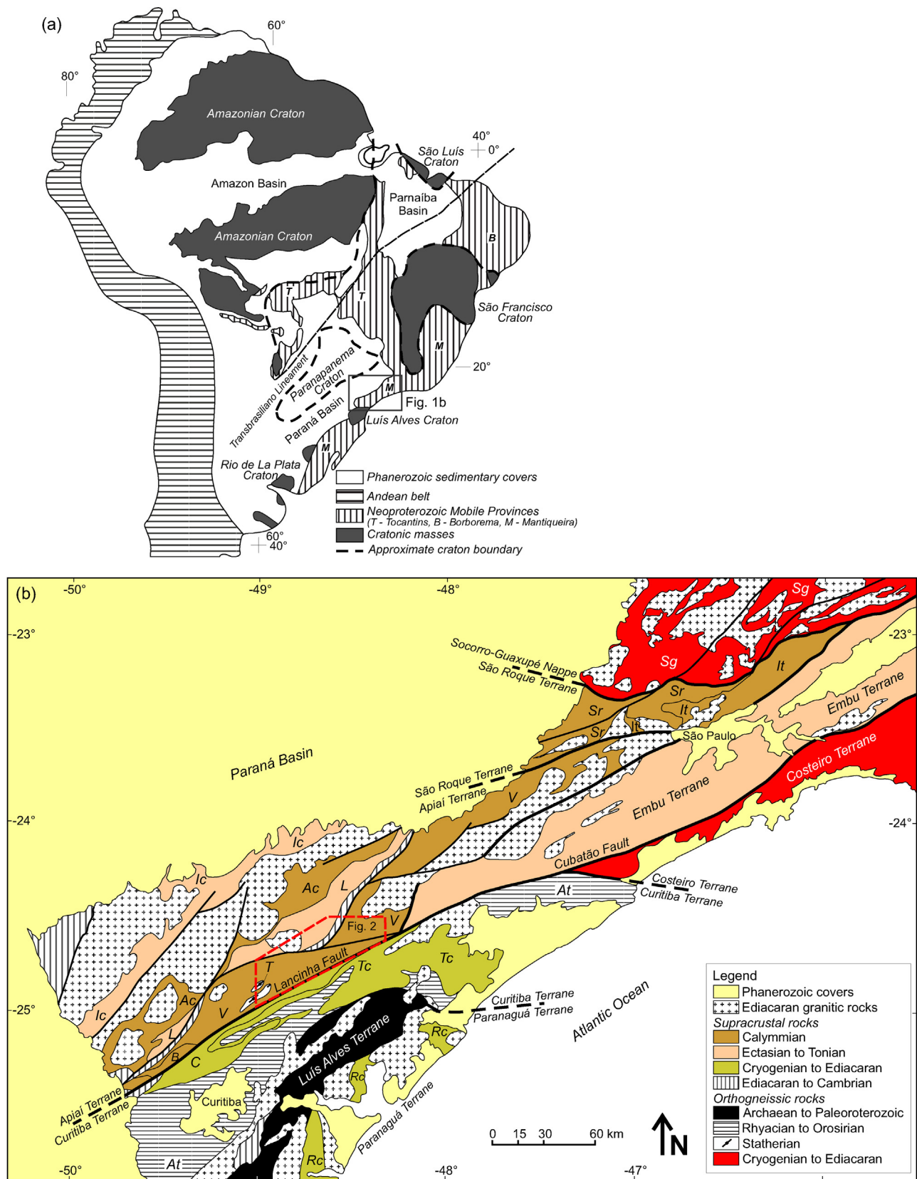
Fig. 1. (a) Simplified geotectonic map of part of South America emphasizing cratonic areas and mobile belts (relative to the Neoproterozoic). (b) Simplified geological map of the southern and central portions of the Ribeira Belt with the location of Fig. 2. Geological units: Itaiaococa Group (Ic), Água Clara Formation (Ac), Lajeado Group (L), Votuverava Group (V), Betara Formation (B), São Roque Group (Sr), Serra do Itaberaba Group (It), Socorro-Guaxupé Nappe (Sg), Tigre Gneiss (T), Capiiru Formation (C), Turvo-Cajati Formation (Tc), Rio das Cobras Formation (Rc), Atuba Complex (At).
