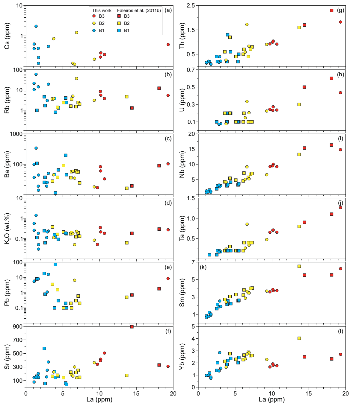
Fig. 11. Plots of La versus LILE (Cs, Rb, Ba, K 2 O, Pb, Sr) (a–f) and HFSE (Th, U, Nb, Ta, Sm, Yb) (g–l) contents.
