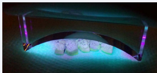
Figure 2 Bleaching process with light irradiation on bovine teeth associated to hydrogen peroxide (35% v/v).
