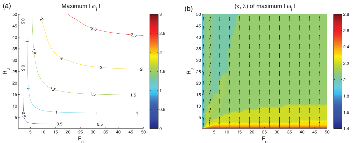
Figure 7. The same as Figure 6, except that the results are for the AL scheme rather than the een scheme.
