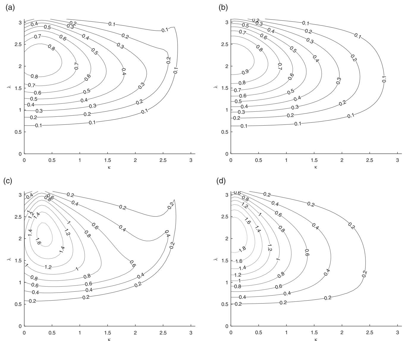
Figure 5. The fastest growing instabilities (maximum |\omega_i| ) for varying \lambda and \kappa for the original een scheme in height coordinates for the case with v_1 = 0 and four combinations of R_u and F_u . (a) R_u = F_u = 10 . (b) R_u = 10, F_u = 40 . (c) R_u = 40, F_u = 10 . (d) R_u = 40, F_u = 40 .
