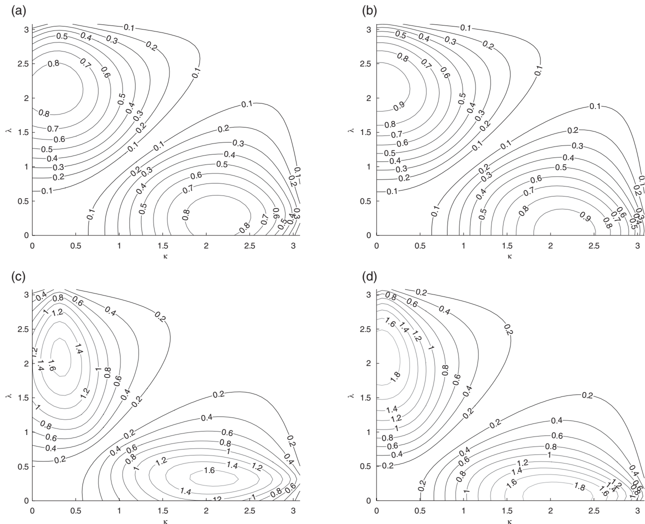
Figure 8. The same as Figure 5 except that instead of v_1 = 0, v_1 = u_1 .
