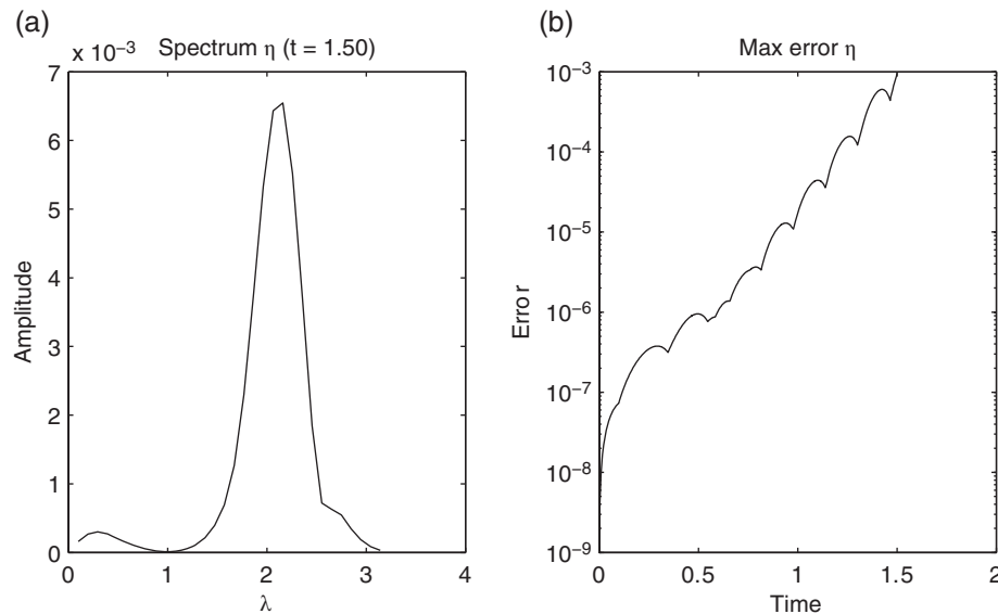
Figure 9. Shallow-water model run with height coordinates, the original een scheme, an initially constant water depth, a constant zonal initial velocity, zonally symmetric forcing to keep the system in a steady state and a small perturbation in the centre of the domain. (a) Spectrum of a y -slice of \eta , where the wave numbers were normalized to (0, \pi) . (b) Evolution of E_\eta(t) , the maximum difference from the initial state of the layer depth \eta .
