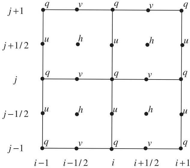
Figure 2. The staggering of variables on the C-grid. This figure and the indexing is based on Arakawa and Lamb (1981).
