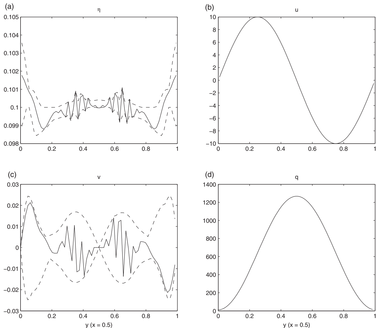
Figure 11. The fields from the same integration as Figure 10 at a time t = 0.35 when the instability is emerging. (a) \eta . (b) u . (c) v . (d) q . In (a) and (c) the middle lines indicate the field values at t = 0.35 and the upper (lower) line indicates the maximum (minimum) value attained earlier in the integration.
