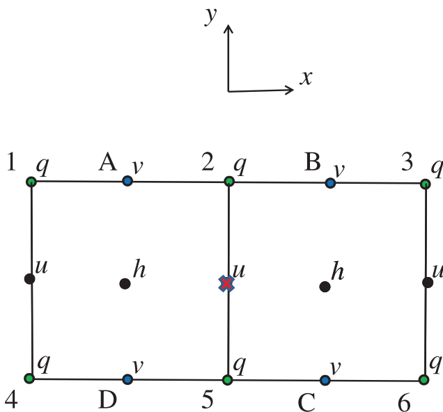
Figure D1. A depiction of the variables used by the een scheme in the calculation of qv^* at the u point in the centre of the figure. The een scheme uses the values of v^* at points A–D and the values of q at points 1–6 at this u point.
