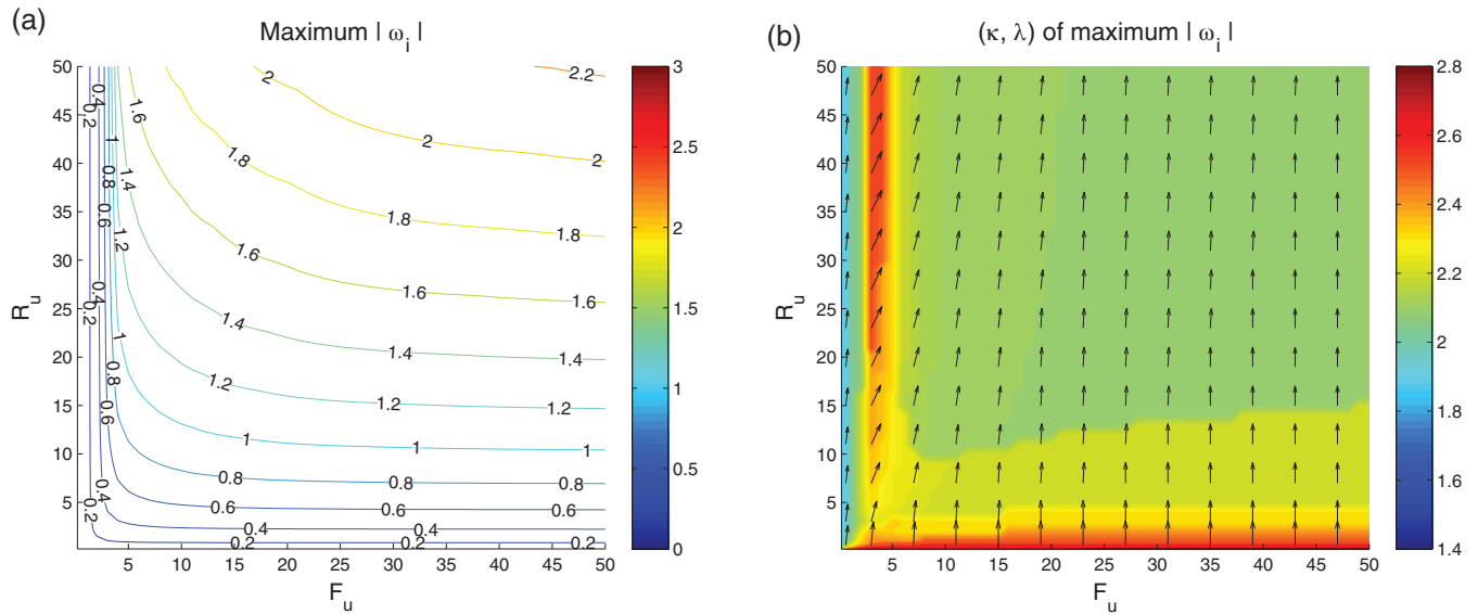
Figure 6. The fastest growing instabilities for all \lambda and \kappa for the original een scheme in height coordinates for the case with v_1 = 0 as a function of F_u (on the abscissa) and R_u : (a) the maximum growth rates \omega_i and (b) their wave number (\kappa, \lambda) ; the arrows show their direction and the contours their magnitude.
