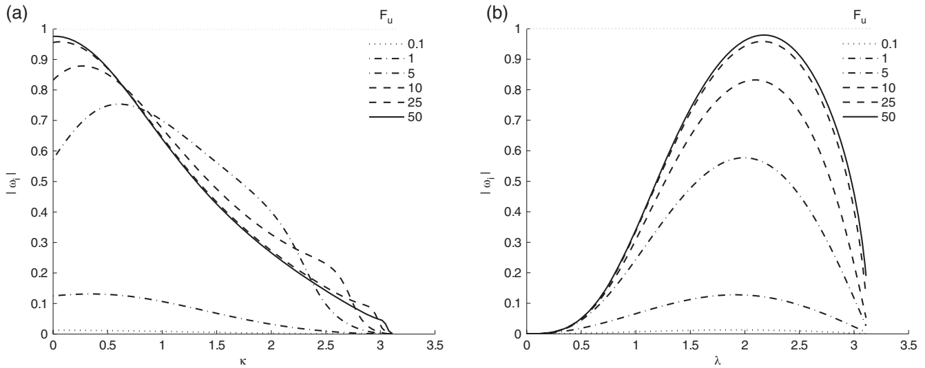
Figure 3. Growth rates, \omega_i , for the original een scheme using height coordinates for a flow aligned with the grid ( v_1 = 0 ), X = 1 and R_u = 10 as functions of (a) \kappa with \lambda = 2\pi/3 and (b) \lambda with \kappa = 0 .
