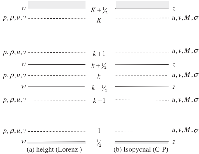
Figure 1. The arrangement of variables using (a) height coordinates and (b) isopycnal coordinates. In both grids, u and v are held at full levels and the upper and lower boundaries are at half-levels.
