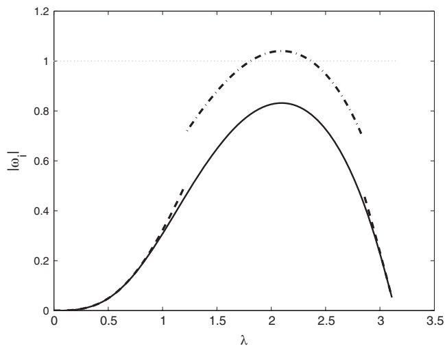
Figure 4. Growth rates, \omega_i , for the original een scheme using height coordinates for a flow aligned with the grid ( v_1 = 0 ), X = 1 , R_u = 10 and F_u = 10 as functions of \lambda with \kappa = 0 . Solid line: (72). Dash-dotted line: (88). Dashed line: (89).
