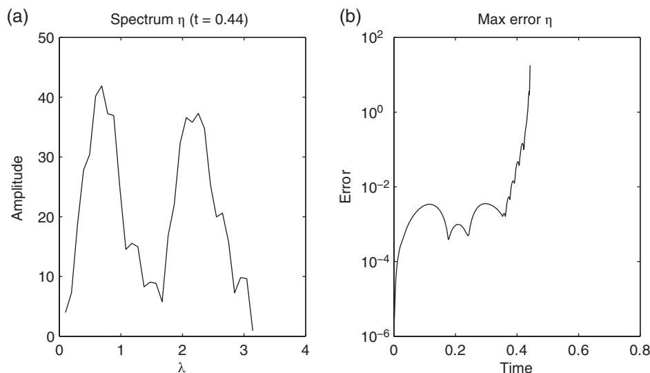
Figure 10. Shallow-water model run with height coordinates, the original een scheme, an initially constant water depth and sinusoidal zonal velocity with a bottom topography, which keeps the zonal flow in balance. (a) Spectrum of a y -slice of \eta , where the wave numbers were normalized to (0, \pi) . (b) Evolution of E_\eta(t) , the maximum difference from the initial state of the layer depth \eta .
