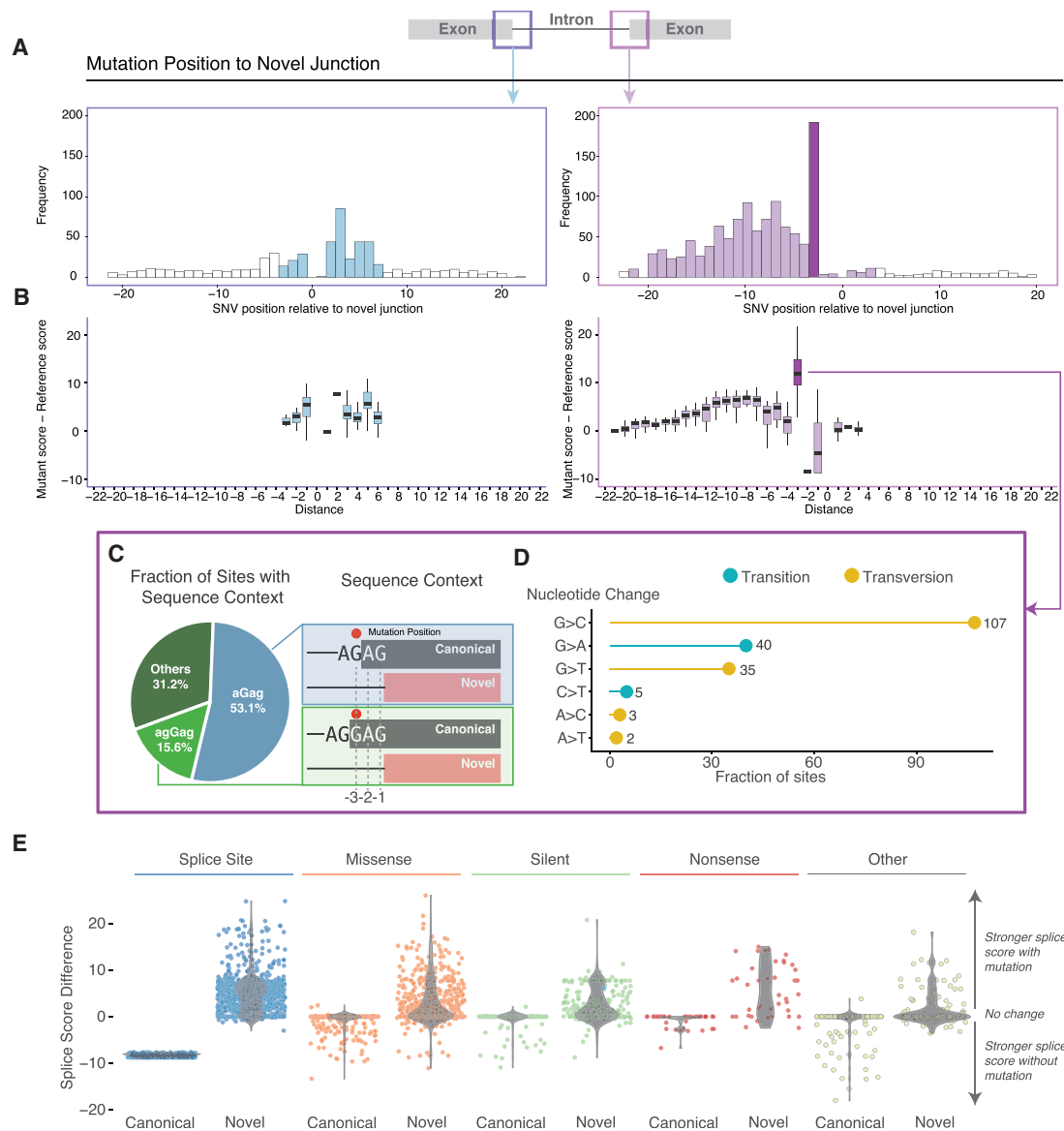
Figure 2. Sequence Contexts and Characteristics of Splice-Site-Creating Mutations
