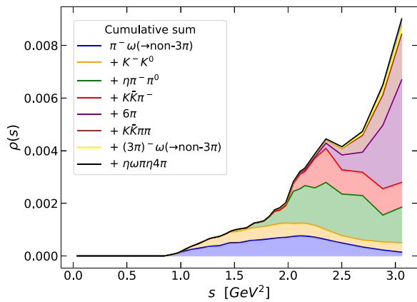
FIG. 4. Residual modes contributions to the spectral function. Left panel: individual modes; right panel: cumulative residual-mode sums.
