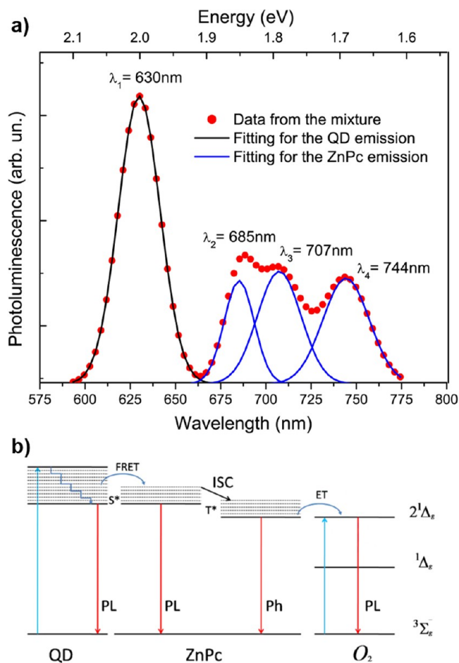
Figure 12. Photoluminescence spectra of CdSe/ZnS-ZnPc (a). The multipeak Gaussian fitting shows four emission peaks from QDs (630 nm), ZnPc (685 and 744 nm), and ^1\text{O}_2 (707 nm). Jablonski energy diagram representation of energy transfer from QDs to ZnPc and ground state molecular oxygen, producing ^1\text{O}_2 : PL (photoluminescence), ISC (intersystem crossing), Ph (phosphorescence), and ET (energy transfer). Reproduced with permission from ref 71. Copyright 2020, Wiley-VCH.
