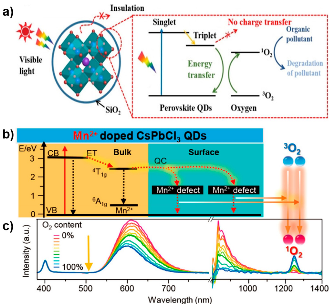
Figure 17. Suggested mechanism for excitonic processes of silica-coated Cs 3 PbBr perovskite QDs and the subsequent energy transfer to the oxygen ground state (a). Reproduced with permission from ref 61. Copyright 2019, Wiley-VCH. The proposed mechanism of Mn 2+ -doped CsPbCl 3 for 1 O 2 generation in which exciton-activated Mn 2+ transferred its energy to two surface Mn 2+ defect states subsequently sensitizing 1 O 2 generation (b). Gradual decline in the luminescence intensities of Mn 2+ at 610 nm and defect at 950 nm and the concomitant increase in phosphorescence intensity of 1 O 2 at 1270 with increasing oxygen content (c). Reproduced with permission from ref 68. Copyright 2020, American Chemical Society.
