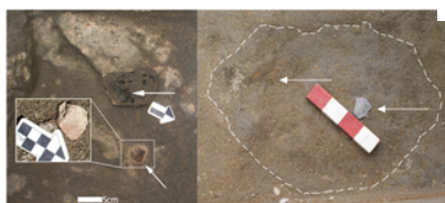
Fig 3. Excavated archaeological features.
