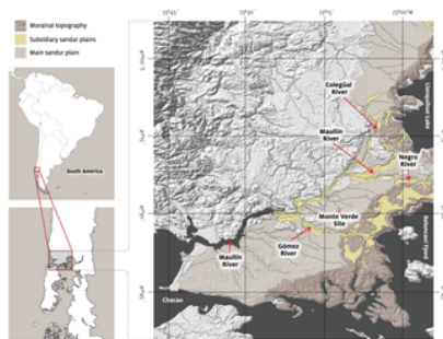
Fig 1. Geomorphological context of the Monte Verde site within the wider context of the Llanquihue drift.
