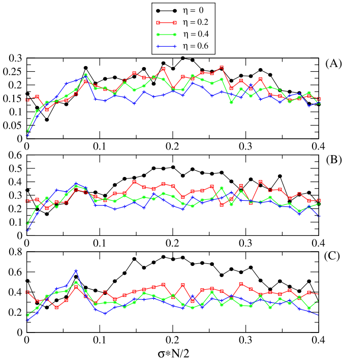
Fig. 5. We show the value of \Lambda as a function of the rescaled coupling strength \frac{\sigma N}{2} . From (A) to (C) we show results concerning networks with N = [10, 20, 30] . Filled circles represent \eta = 0 , empty squares \eta = 0.2 , stars \eta = 0.4 , and pluses \eta = 0.6 .
