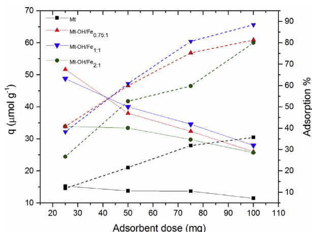
Figure 7. Effect of the dose of adsorbent on the adsorption of phosphate. Experiments made with phosphate initial concentration of 323 \mu\text{mol L}^{-1} (10 mg \text{L}^{-1} in P) at 25.0 \pm 0.5^\circ\text{C} , contact time = 180 min, initial pH = 6.90 \pm 0.05 .
