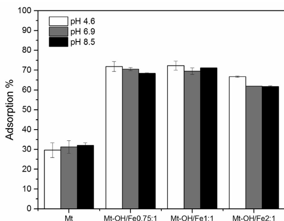
Figure 10. Influence of the initial pH on the adsorption of phosphate from a 484 \mu\text{mol L}^{-1} solution ( 15 \text{ mg L}^{-1} in P) using 100 mg of adsorbent dispersed in 10.0 mL of solution and 180 min of contact time at 25.0 \pm 0.5 °C.
