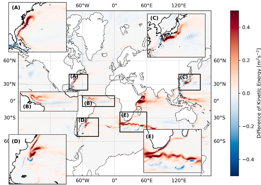
Fig. 14. Kinetic Energy difference between a reference simulation and simulation without the use of biharmonic, i.e. E_k^{(ref)} - E_k^{(no\ bih)} .
