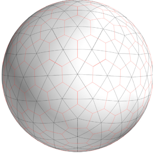
Fig. 1. SCVT primal (black lines) and dual (red lines) g_2 grid.
