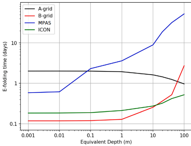
Fig. 11. E-folding time for the different evaluated schemes, considering a time-step of 200 s in a geostrophic test case where the balanced state is given by the bathymetry, while the height is given by the equivalent depth and constant.
