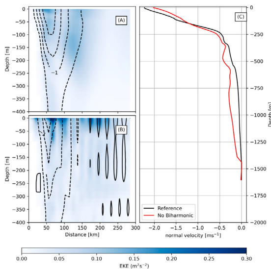
Fig. 17. P1 Cross-section between the Reference simulation (A), and No Biharmonic Simulation (B), and the vertical profile of the normal velocity in the 42 km distance (C).
