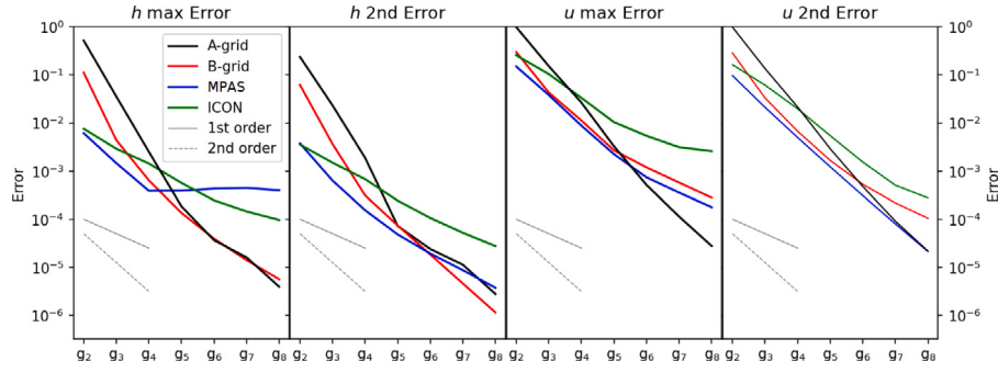
Fig. 6. h and u error after 15 days.
