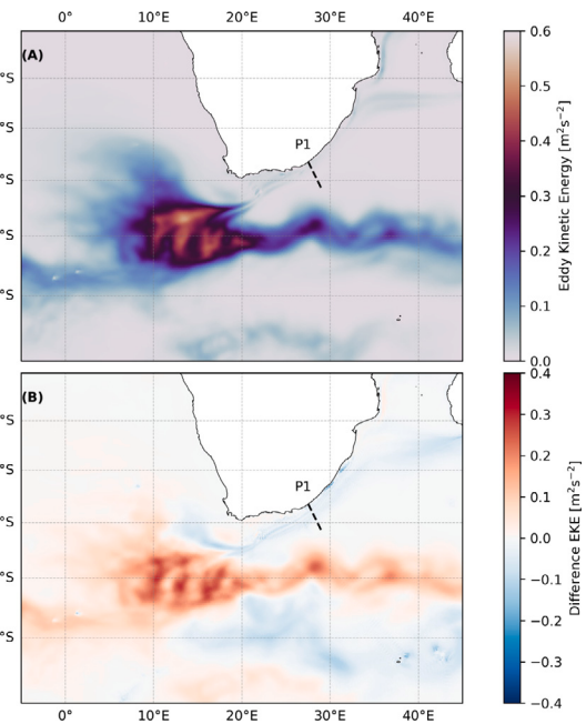
Fig. 16. Eddy Kinetic Energy (A) and the difference between simulations of EKE (B) of the Agulhas Current System.
