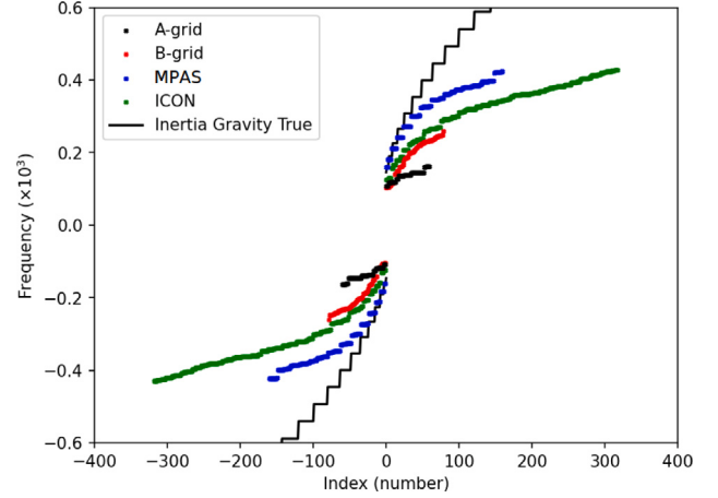
Fig. 7. Linear normal modes of the considering the linear shallow water Eqs. (23) on the f -sphere.
