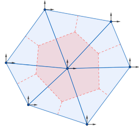
Fig. 2. A-grid cell structure. The blue circles on the vertices are the height scalar points, and the arrows are the components of the velocity vector points.
