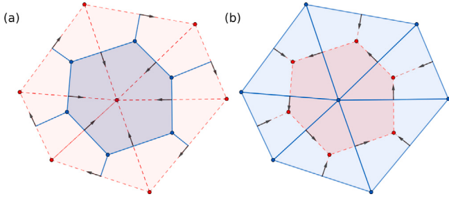
Fig. 4. C-grid cell structure, considering hexagons (a) and triangles (b) as the primal grid. Red circles are the height scalar points, and the arrows are the decomposed velocity vector field.
