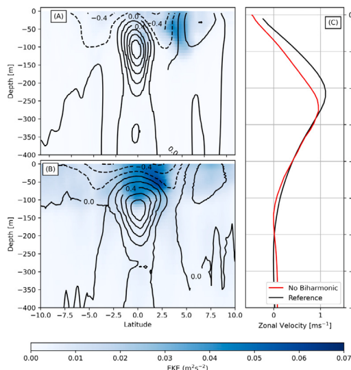
Fig. 15. Cross-section of the 130°W longitude of the reference (A) and the without biharmonic (B) simulation, and a vertical profile of the zonal velocity of both simulations over the 0° Latitude (C).
