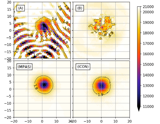
Fig. 8. Height field of the different schemes for the localized balanced flow testcase without using biharmonic for both A- and B-grid schemes. Using a grid refinement g_6 and a timestep of 50 s.
