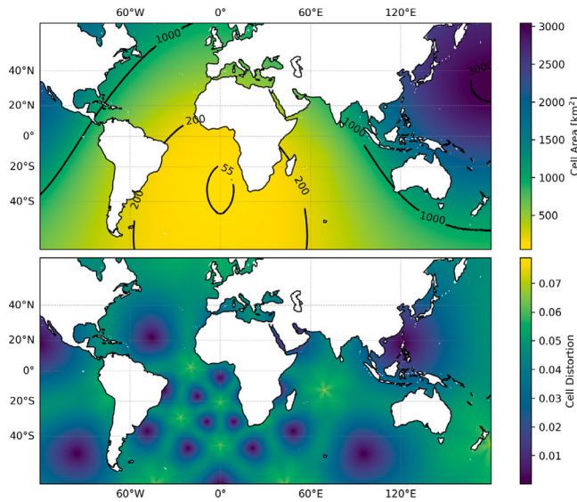
Fig. 13. The upper panel is the cell area of the spherical grid used in the simulations. The lower panel is the respective cell distortion of the mesh.
