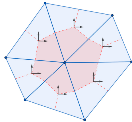
Fig. 3. B-grid cell structure. The blue circles on the vertices are the height scalar points, and the arrows on the triangle centre are the components of the velocity vector points.
