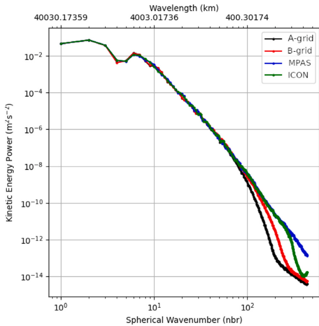
Fig. 10. Kinetic energy spectra for the Barotropic instability testcase for all schemes as in Fig. 9.
