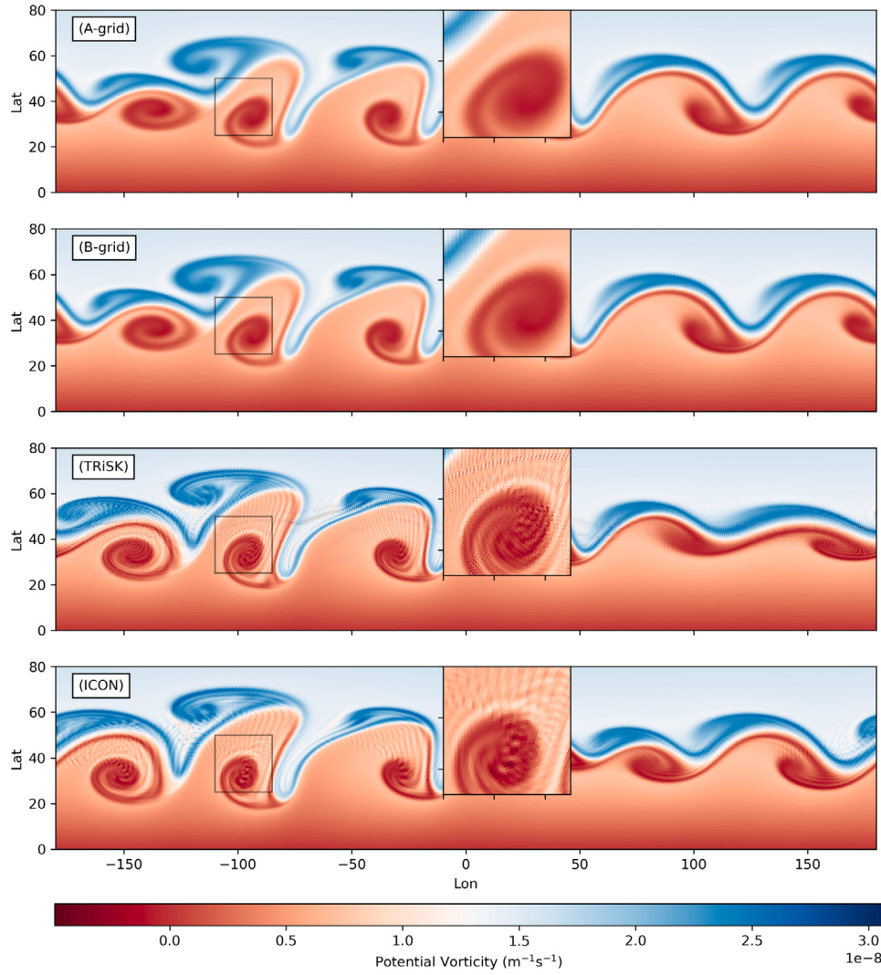
Fig. 9. Potential Vorticity of all schemes on the 6th day of integration for the barotropic instability testcase with perturbation using a g_7 refinement grid and a respective biharmonic for A- and B-grid schemes, following Table 4.
