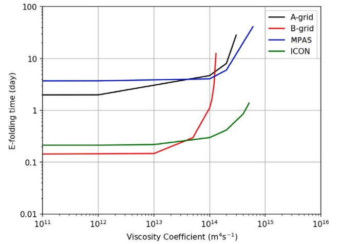
Fig. 12. E-folding time by viscosity coefficient for each scheme, using a g_0 grid refinement with a timestep of 200 s and a 1 m equivalent depth.
