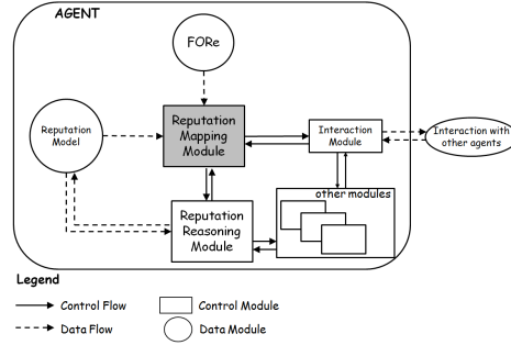
Fig. 1. Agent architecture for reputation interaction
