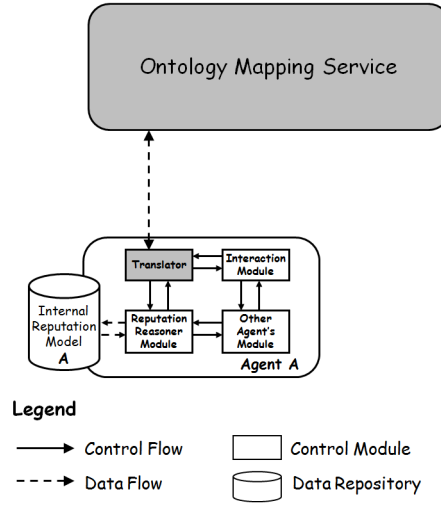
Fig. 2. The proposed service-oriented architecture
