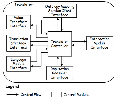
Fig. 4. The Translator Module components
