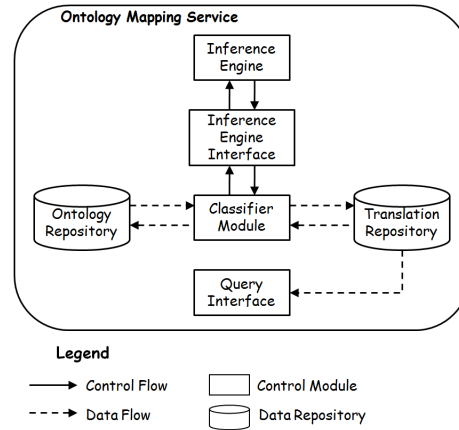
Fig. 3. The Ontology Mapping Service components
