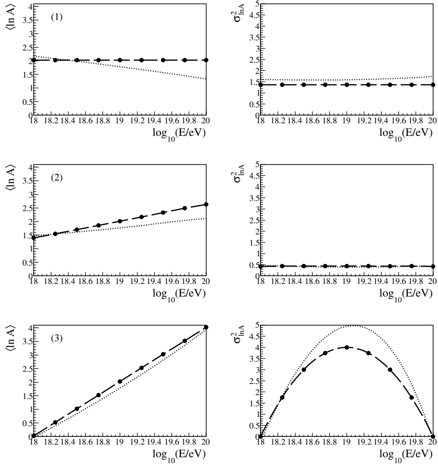
Figure 2. \langle \ln A \rangle and \sigma^2_{\ln A} as a function of \log_{10}(E/\text{eV}) for three different mass distribution hypotheses. Sibyll 2.1 is the hadronic interaction model. Full circles refer to the values obtained directly from the input mass distributions. The dashed lines show \langle \ln A \rangle and \sigma^2_{\ln A} calculated using equations (2.10) and (2.13). The dotted lines refer to the calculation of the same variables using the parameterization for QGSJet II in (2.10) and (2.13).
