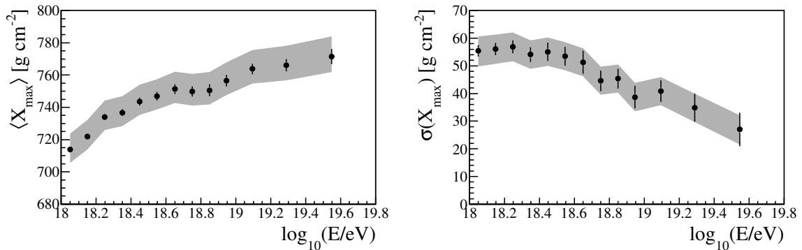
Figure 3. \langle X_{\text{max}} \rangle (left) and \sigma(X_{\text{max}}) (right) as a function of \log_{10}(E/\text{eV}) from Pierre Auger Observatory data [6, 22]. Data (full circles) are shown with statistical errors. Systematic uncertainties are represented as bands.
