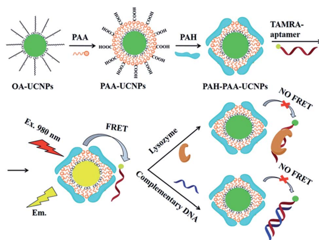
Fig. 14 Schematic illustration of the synthesis steps and working principle of the 1RFS FRET biosensor for lysozyme and DNA detection based on ppUCNP-TAMRA nanoprobos. Reprinted with permission from ref. 171. Copyright 2015, The Royal Society of Chemistry.
