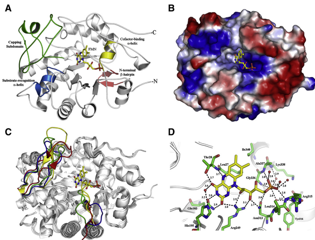
Fig. 2. TcOYE structural analysis. A) Overall fold highlighting the extra barrel elements and the FMN prosthetic group. B) Electrostatic surface representation with the FMN molecule bound to the active-site pocket. The positively charged regions are indicated in blue and the negatively charged regions are indicated in red. C) Structural superposition of TcOYE structure (green) on OYEs from Burkholderia pseudomallei (blue), Shewanella oneidensis (yellow) and Solanum lycopersicum (red). The structurally distinct regions are colored according to the protein. D) A zoom of the FMN binding site showing all contacts established between TcOYE and FMN.
