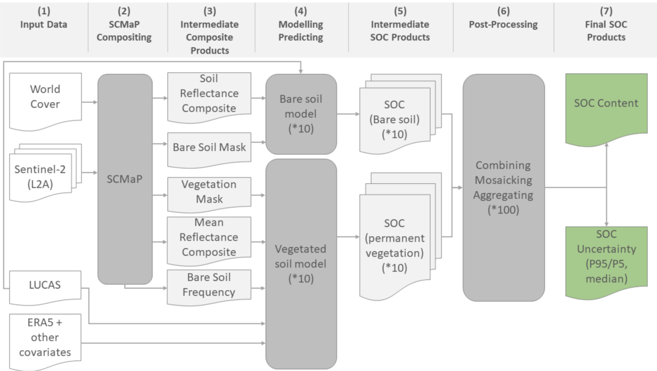
Fig. 1. Flowchart of the SOC monitoring system to derive topsoil SOC content at continental scale. The number in brackets indicates the number of iterations and resulting products with P5 and P95 being the 5th and 95th percentile.
