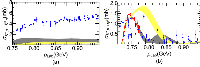
FIG. 2. A comparison of the cross sections obtained with (dark shaded) and without (light shaded) the coupling of pseudoscalar-baryon channels to vector-baryon channels.
