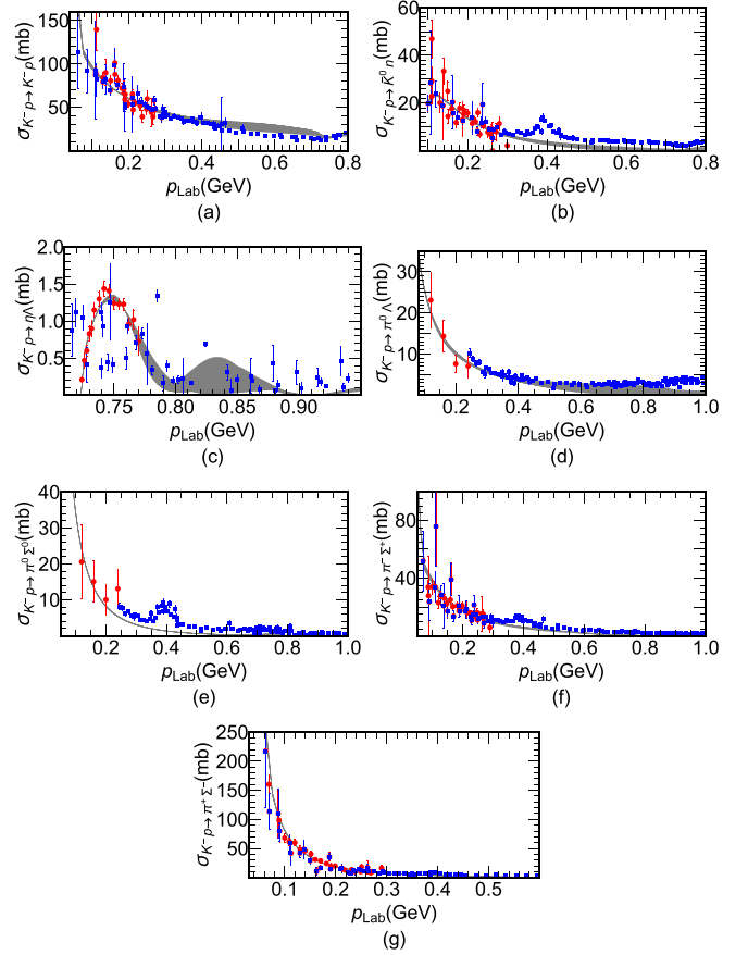
FIG. 1. Cross sections of different processes studied in our work. The shaded region represents the results found with the parameters listed under the label Fit I in Table I. Data shown as (red) filled circles (taken from Refs. [61–67]) were used in the \chi^2 fitting procedure explained in the text.
