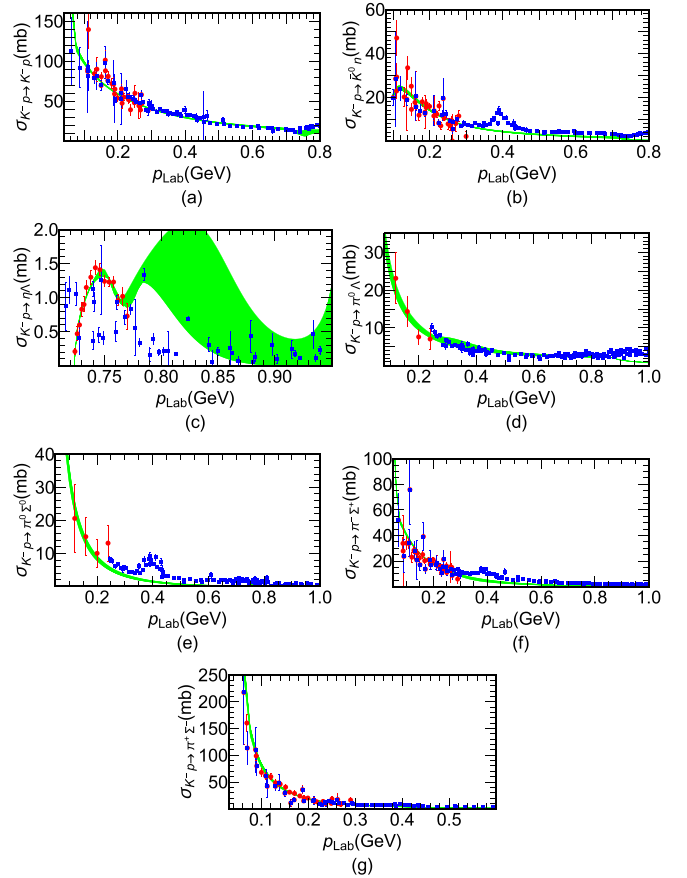
FIG. 3. Cross sections obtained with the parameter set Fit II given Table I. The data are taken from the same source as in Fig. 1.
