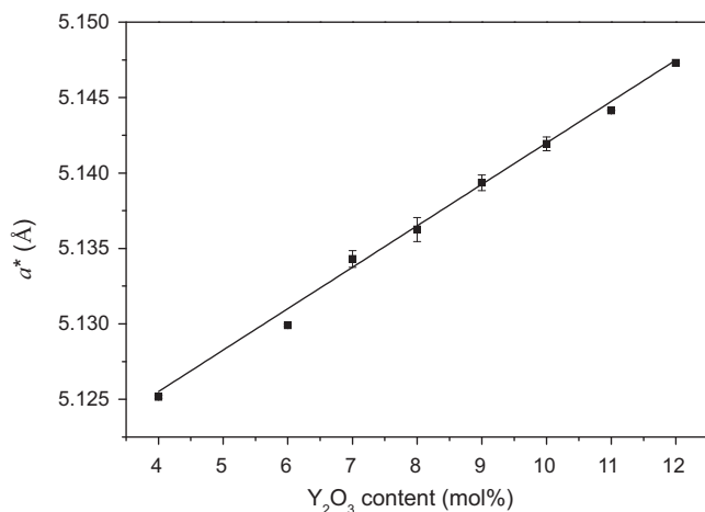
Fig. 7. Pseudo-cubic lattice parameter, a^* = (2a + c)/3 , as a function of Y 2 O 3 content. The solid line is a linear fit of the experimental results.
