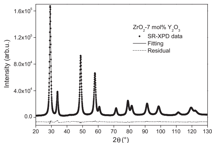
Fig. 1. Experimental SXPD data and fit obtained after Rietveld refinement assuming one tetragonal phase for the \text{ZrO}_2 -7 mol% \text{Y}_2\text{O}_3 sample.
