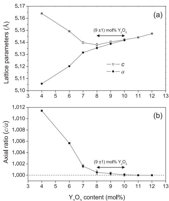
Fig. 2. Variation of the lattice parameters, a and c , and the axial ratio, c/a , as functions of \text{Y}_2\text{O}_3 content. The t'/t'' compositional boundary at (9 \pm 1) mol% \text{Y}_2\text{O}_3 is indicated with arrows.
