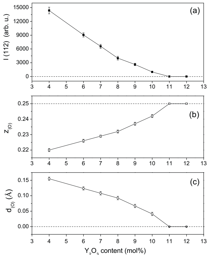
Fig. 4. (a) Integrated intensity of the 1 1 2 Bragg reflection, (b) z_{(0)} fractional coordinate and (c) d_{(0)} distance, as functions of \text{Y}_2\text{O}_3 content. See text for details.
