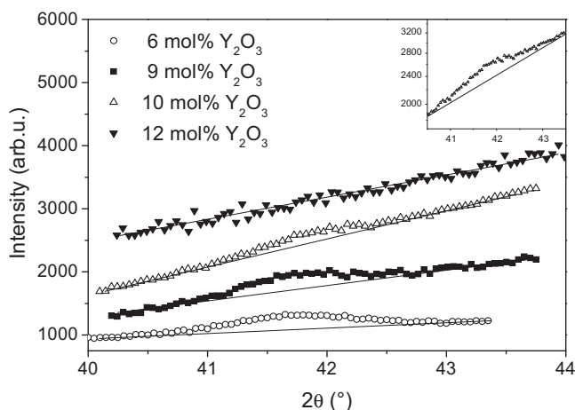
Fig. 3. SXPD data close to the 1 1 2 Bragg reflection for the \text{ZrO}_2 -6, 9, 10 and 12 mol% \text{Y}_2\text{O}_3 solid solutions, taken with step-counting times of 12 s, 15 s, 30 s and 30 s, respectively. All data were normalized considering these different step-counting times. The inset shows the \text{ZrO}_2 -10 mol% \text{Y}_2\text{O}_3 sample in more detail. The straight lines are a guide for the visualization of the background.
