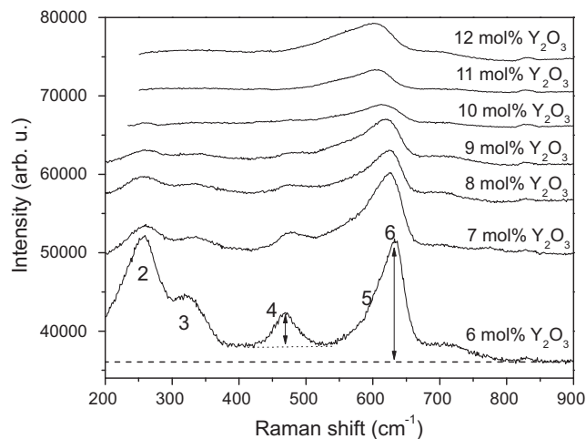
Fig. 5. Raman spectra of \text{ZrO}_2 - \text{Y}_2\text{O}_3 solid solutions. The numbers correspond to the bands mentioned in the text and in Ref. [4]. The dotted line is the background estimation for the fourth band while the dashed line corresponds to the sixth one.
