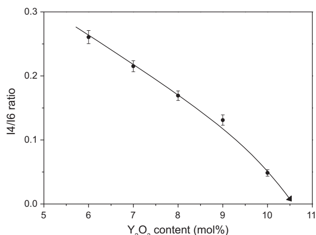
Fig. 6. 14/16 peak height ratio derived from Raman spectroscopy analysis, as functions of Y 2 O 3 content. The solid line is a guide to the eye.
